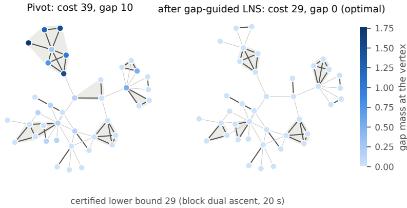
Fig. 3 Gap decomposition (Theorem 7) on the neighbourhood of Figure 2. Each vertex is coloured by its share of \text{cost}(\mathcal{C}) - \text{LB} (pair terms split between the endpoints, row terms between the vertices of the row); shaded regions are clusters, dark edges lie inside a cluster. Left: a Pivot clustering. Right: after gap-guided LNS the gap is zero, so the clustering is optimal. Computed by the released code.
