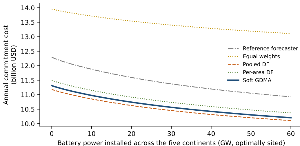
Figure 8: Annual system-wide commitment cost as a function of battery power installed and optimally sited across the 125 grid areas, for five commitment rules. Costs valued at $10 per MWh of idle committed capacity; annual values average over each area’s own evaluation period. Lower is better.
