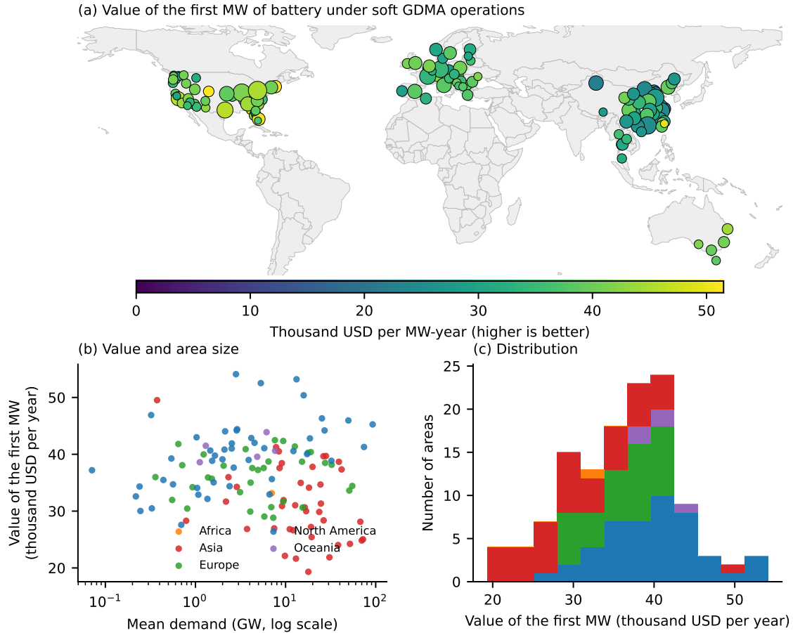
Figure 7: Where batteries are worth most when operations follow soft GDMA: value of the first MW of battery power in each area (higher is better), against the area's size and its distribution.
