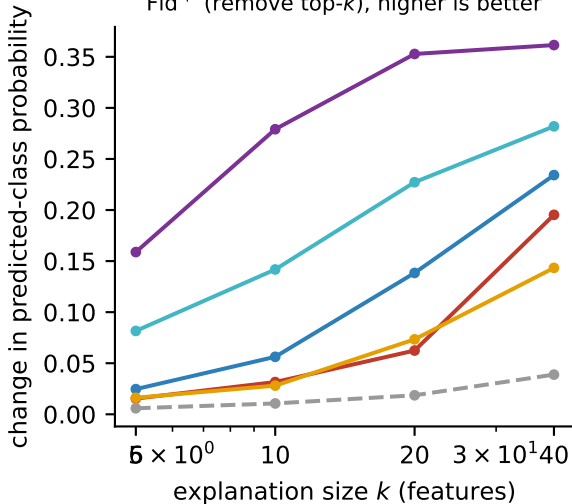
Fid + (remove top- k ), higher is better
