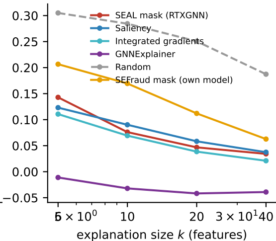
Fid - (keep only top- k ), lower is better
