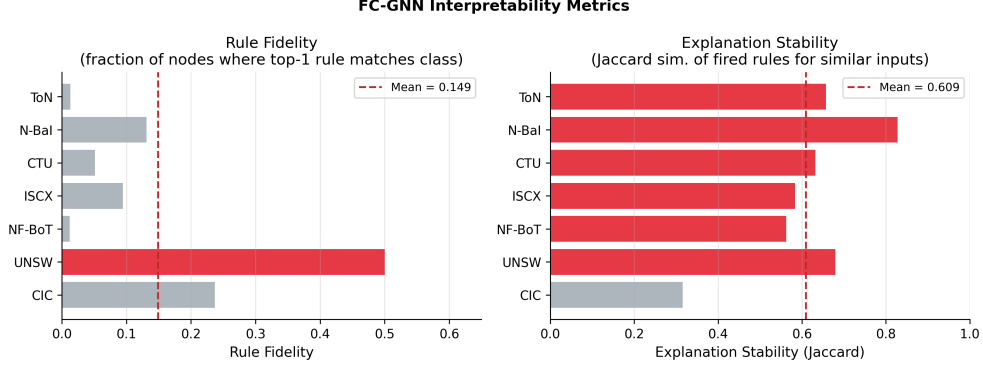
Fig. 7: FC-GNN interpretability metrics across seven cybersecurity datasets. Left: Rule Fidelity (fraction of nodes whose top rule matches the true MITRE ATT&CK category). Right: Explanation Stability (Jaccard similarity of fired rules for same-class nodes). Red dashed lines = dataset means.
