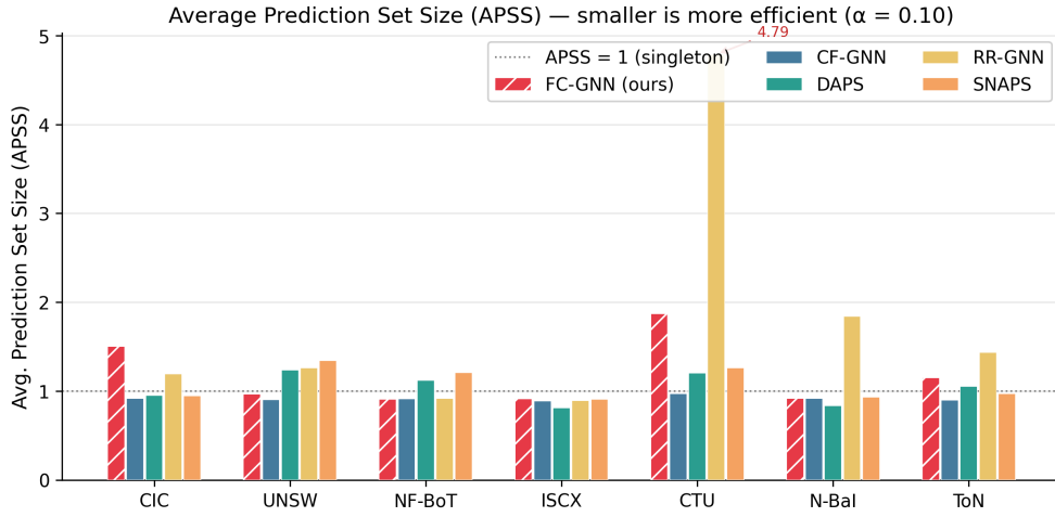
Fig. 3: Average Prediction Set Size (APSS, lower is more efficient). FC-GNN is significantly more efficient than RR-GNN on CTU-13 (1.87 vs 4.79, annotated).
