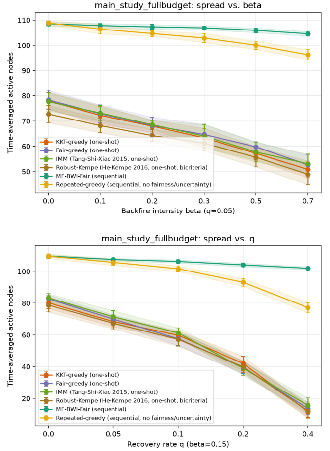
Fig. 1. Full sweeps underlying Table I (mean \pm 95% CI shading, 15 trials per point): time-averaged spread vs. backfire intensity \beta at q = 0.05 (top) and vs. recovery rate q at \beta = 0.15 (bottom), all six algorithms. Both sweeps show the same shape reported in the text at the three extreme points: MF-BWI-Fair statistically tied with repeated-greedy at the low end and opening a significant, growing lead as either parameter increases, with the four one-shot baselines clustered well below both throughout.
