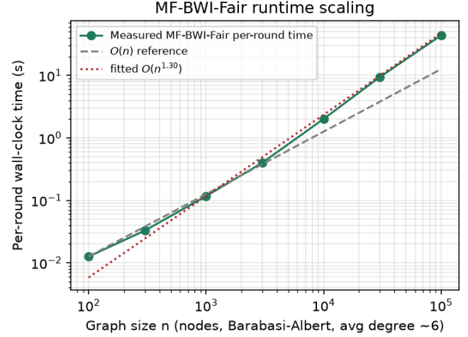
Fig. 2. MF-BWI-Fair per-round wall-clock time vs. graph size n (Barabasi-Albert, average degree \approx 6 , log-log axes), against an O(n) reference line and the fitted O(n^{1.30}) power law.
