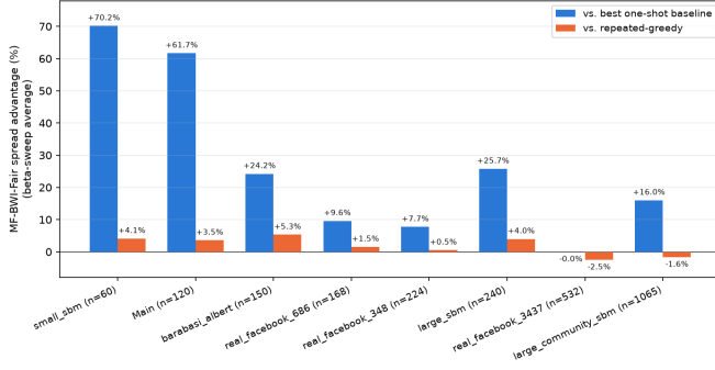
Fig. 5. MF-BWI-Fair’s mean spread advantage (%) over the best one-shot baseline and over repeated-greedy, averaged across each graph’s own \beta sweep, for all eight graphs tested (synthetic and real, ordered by node count).
