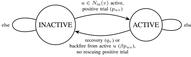
Fig. 1. Per-node round transition, illustrated for a single active in-neighbor u (the full rule, Eq. (1), depends jointly on every active in-neighbor: any one successful positive trial rescues or activates v , overriding recovery/backfire that same round).
