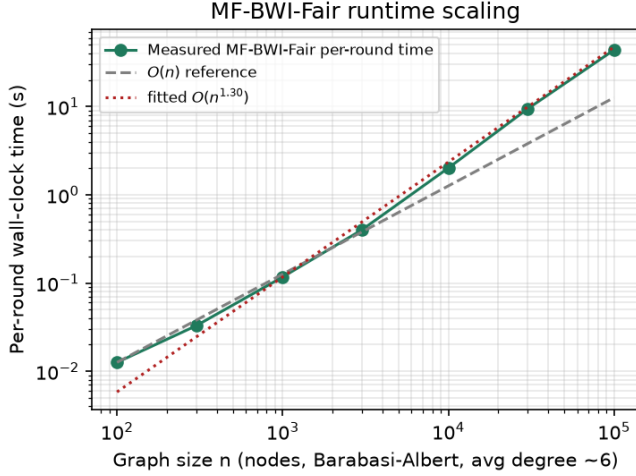
Fig. 4. MF-BWI-Fair per-round wall-clock time vs. graph size n (Barabasi-Albert, average degree \approx 6 , log-log axes), against an O(n) reference line and the fitted O(n^{1.30}) power law.
