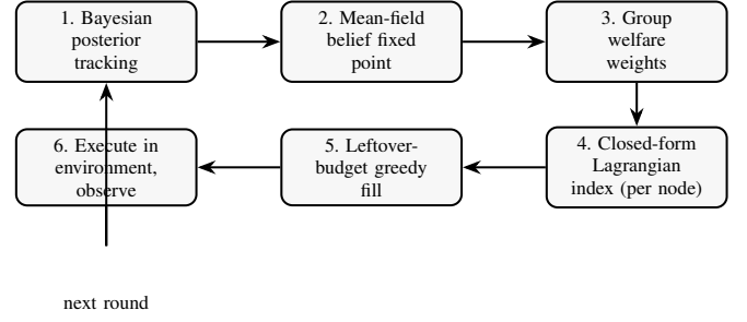
Fig. 2. MF-BWI-Fair’s per-round control loop (numbered as in the list above); Algorithm 1 gives the corresponding pseudocode.
