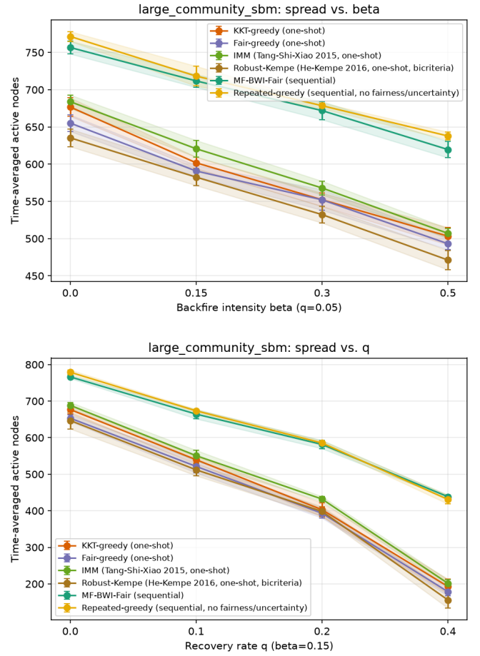
Fig. 6. large_community_sbm (1,065 nodes, six community sizes scaled from real_facebook_3437 ): time-averaged spread vs. backfire intensity \beta at q = 0.05 (top) and vs. recovery rate q at \beta = 0.15 (bottom), mean \pm 95% CI shading, 6 trials per point. MF-BWI-Fair (teal) leads every one-shot baseline throughout and tracks repeated-greedy (yellow) closely, unlike the stable, one-sided gap seen on real_facebook_3437 itself.
