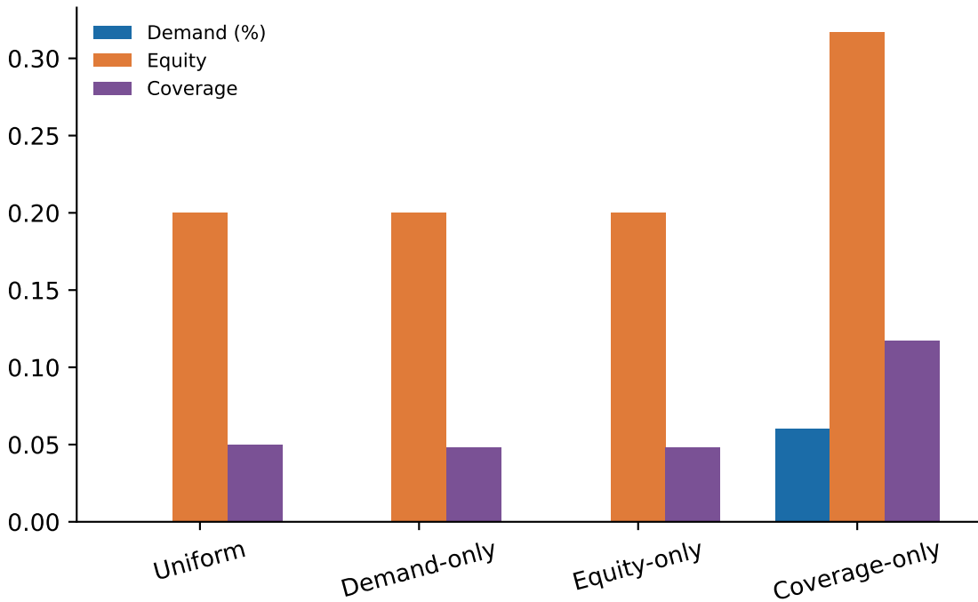
Xi'an \texttt{full} (seed 42): weight-conditioning sanity check
