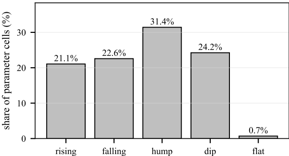
term-structure shape, 139,968 cells
