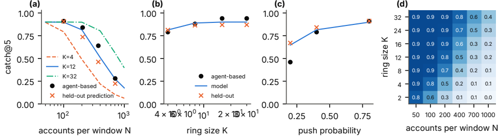
Fig. 3 The scaling law against the agent-based market. (a)–(c) catch@5 against the number of accounts, the ring size and the push probability: points are simulated, lines are the model (8) fitted to all sweeps, crosses are predictions with the plotted sweep held out. (d) Model catch@5 over the number of accounts and the ring size at push probability 0.8
