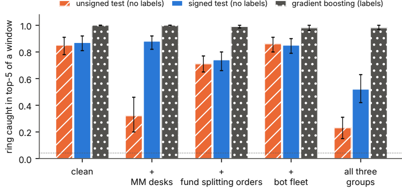
Fig. 4 Share of ring-active windows in which a ring member is among the five top-ranked accounts, with 95% bootstrap intervals over 24 episodes. The dotted line is the chance level. The unsigned test is crowded out by market-making desks; the signed test is not. Gradient boosting is trained with labels on rings in the clean market
