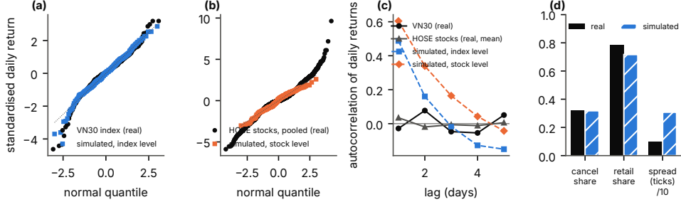
Fig. 1 Calibration of the simulated markets against real data. (a) Standardised daily returns of the VN30 index since 2023 and of the first accepted index-level market, against normal quantiles. (b) Pooled standardised daily returns of 378 HOSE stocks since 2022 and of the first accepted stock-level market. (c) Autocorrelation of daily returns at lags 1 to 5: VN30 index, mean over HOSE stocks, and the first accepted market of each simulated family (pooled over episodes). (d) Cancel share, retail share (midpoint of the published range 0.75–0.82) and spread in ticks divided by 10 (VN30 futures: one tick for 73% of quotes); the simulated spread is not matched
