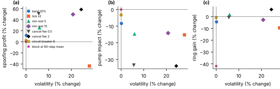
Fig. 10 Effect on manipulators against cost to honest participants, first calibrated market. Each point is an order-level rule or band setting; the horizontal axis is the change of the honest-only volatility, the vertical axis the change in (a) spoofing profit, (b) pump impact and (c) ring gain, relative to the market with a 7% band and no other rule. Manipulators do not adapt
