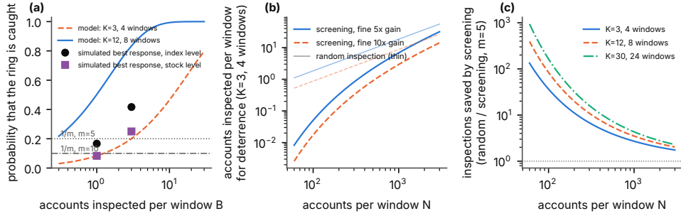
Fig. 9 Deterrence frontier. (a) Probability that the ring is caught against the number of inspected accounts per window at N = 600 for two ring sizes (model, solid and dashed), with the thresholds 1/m for m = 5, 10 (horizontal lines) and the median probability of the best-responding ring in the two simulated families (points). (b) Accounts to inspect per window for deterrence of a ring of three accounts active in four windows against N , by screening (thick) and by random inspection (thin). (c) Inspections saved by screening against N for three ring sizes and activity levels, fine five times the gain
