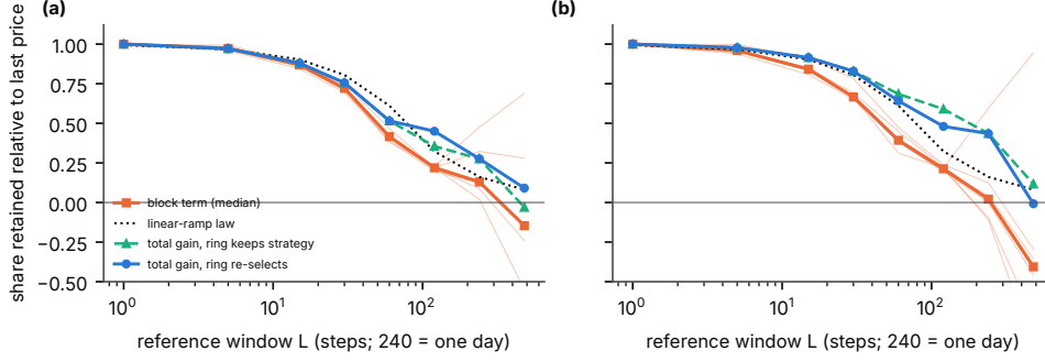
Fig. 8 Share of the ring’s block term and of its total gain retained against the reference window L , for the index-level (a) and stock-level (b) families: median over six markets of the block term (thick orange; thin lines are the six markets), the linear-ramp law of Proposition 6, and the total gain for a ring that keeps its strategy and for a ring that re-selects it
