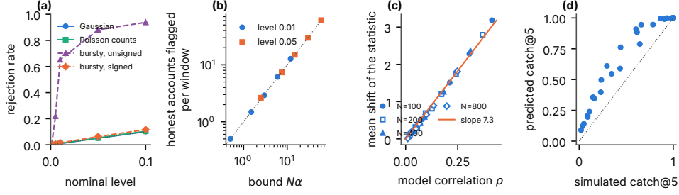
Fig. 2 Monte Carlo checks of the propositions with the implemented test. (a) Rejection rate against nominal level for exchangeable flows (Gaussian, Poisson) and for flows with a shared bursty regime (signed and unsigned variants); dotted line: nominal. (b) Honest accounts flagged per window against the bound N\alpha at levels 1% and 5%. (c) Mean shift of a ring member's statistic against the model correlation \rho of Proposition 3, for N from 100 to 800, k from 4 to 32 and \eta \in \{0.1, 0.3\} ; line: fitted slope. (d) Predicted against simulated catch@5 for the same 32 settings
