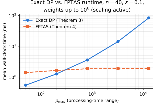
Fig. 4 Table 7 plotted on log-log axes: the exact DP's pseudo-polynomial O(nP) dependence on time grows with p_{\max} (roughly linearly or slightly faster once the fixed overhead is visibly linearly exceeded), while the FPTAS's O(n^3/\epsilon) runtime— independent of p_{\max} — stays flat.
