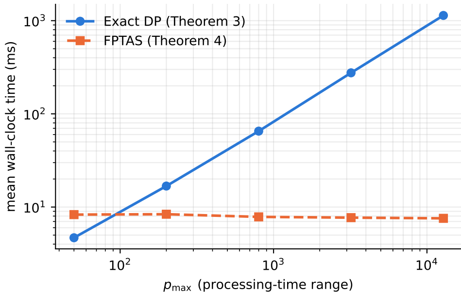
Exact DP vs. FPTAS runtime, n = 40 , \varepsilon = 0.1
