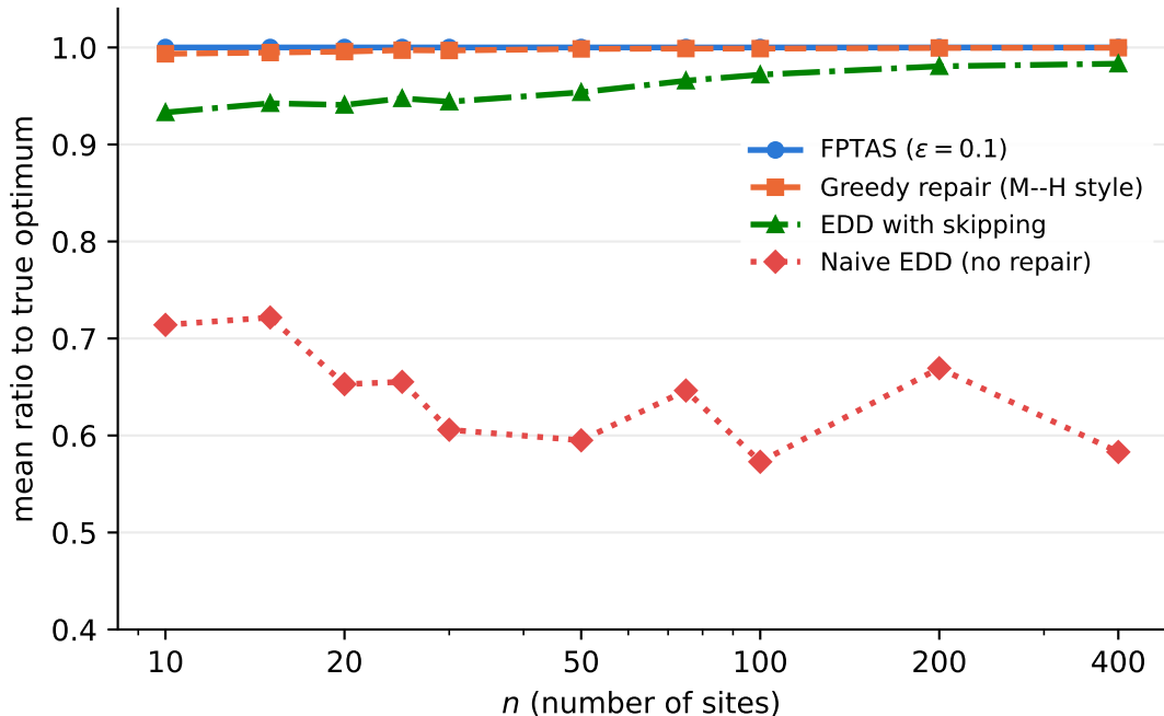
Accuracy across instance sizes (weights \leq 100 )
