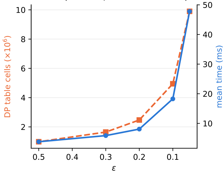
Cost ( n = 100 , random w \leq 10^6 )
