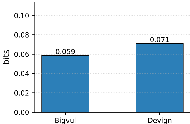
H(\phi \mid \kappa) : information in the taxonomy beyond the grammar kind
