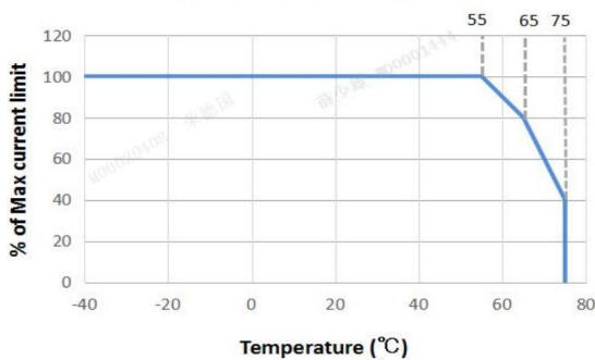
Current limit vs Temperature 176Vac≤Vin≤300Vac
