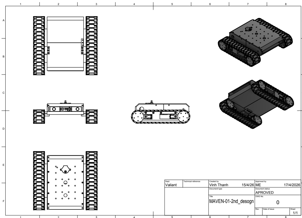
Figure 4: MAVEN-01 second prototype design using separate chassis with chained tracks (Single motor chassis)
