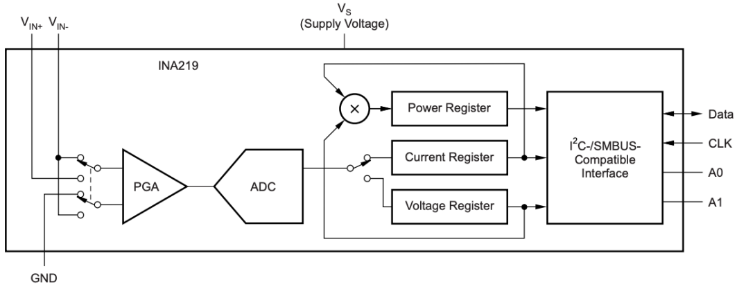
Figure 27: Simplified INA219 Schematic, more information can be found in this datasheet
