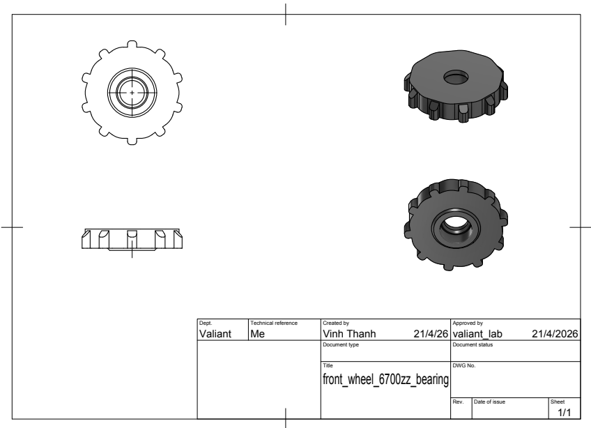
Figure 7: Front wheels with 6700zz bearingblueprint for MAVEN-01
