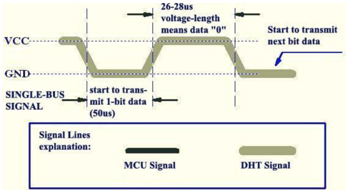
Figure 18: Data "0" Indication
