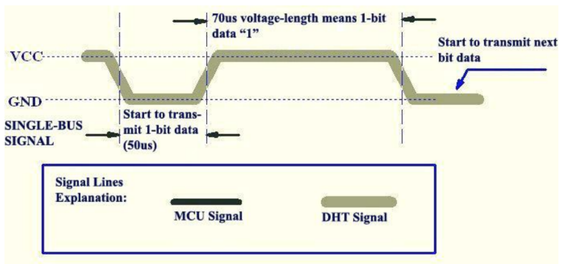
Figure 19: Data "1" Indication
