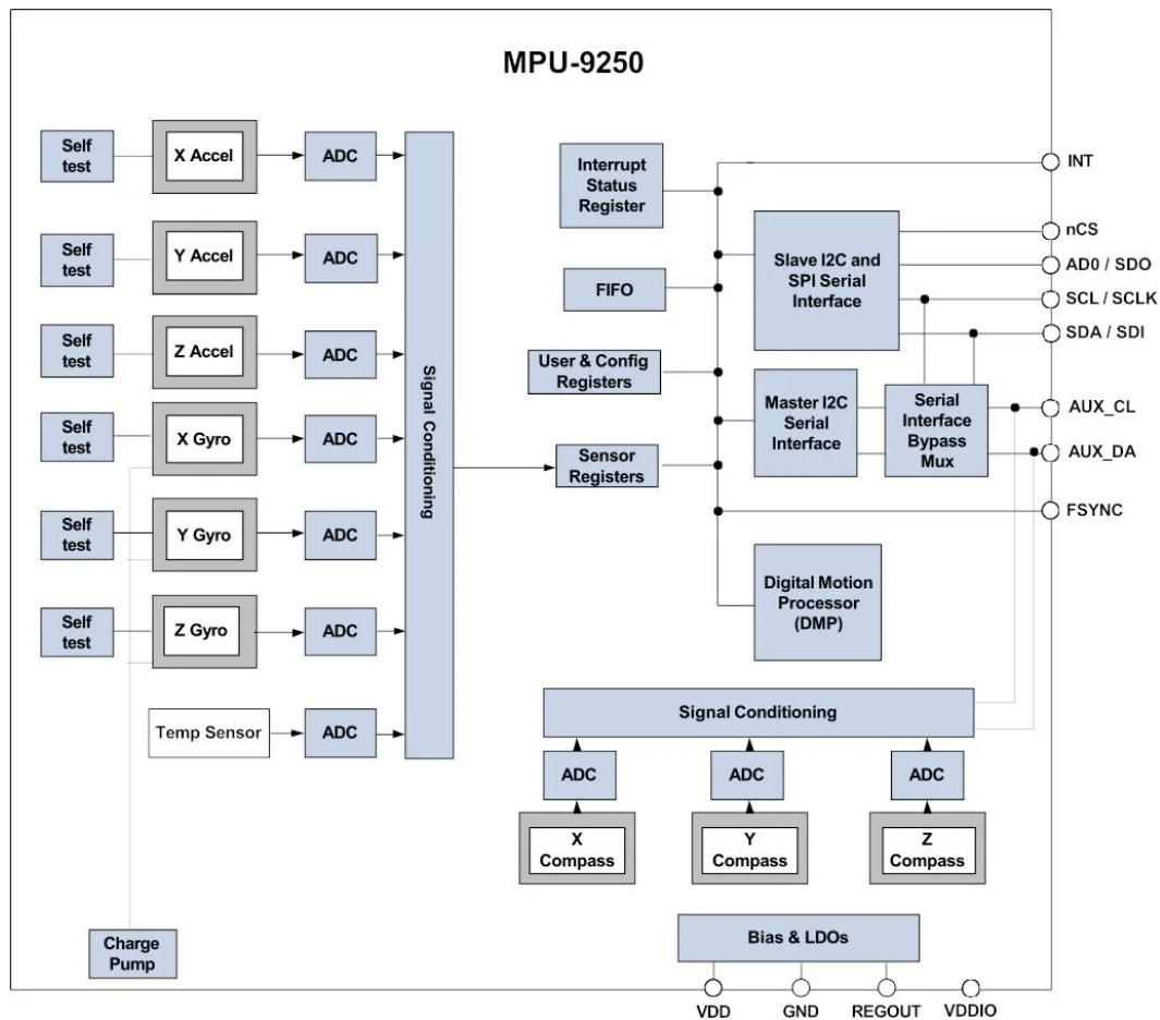
Figure 23: MPU-9250 block diagram, more information can be found in this datasheet , announced by TDK InvenSense
