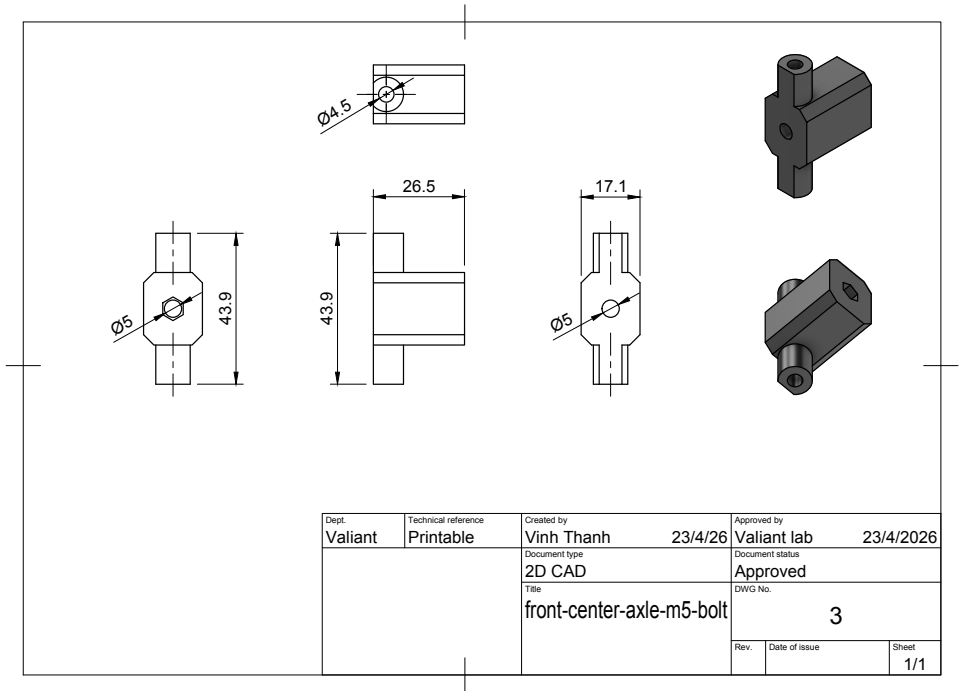
Figure 8: Front axis for front wheels for M5 bolts
