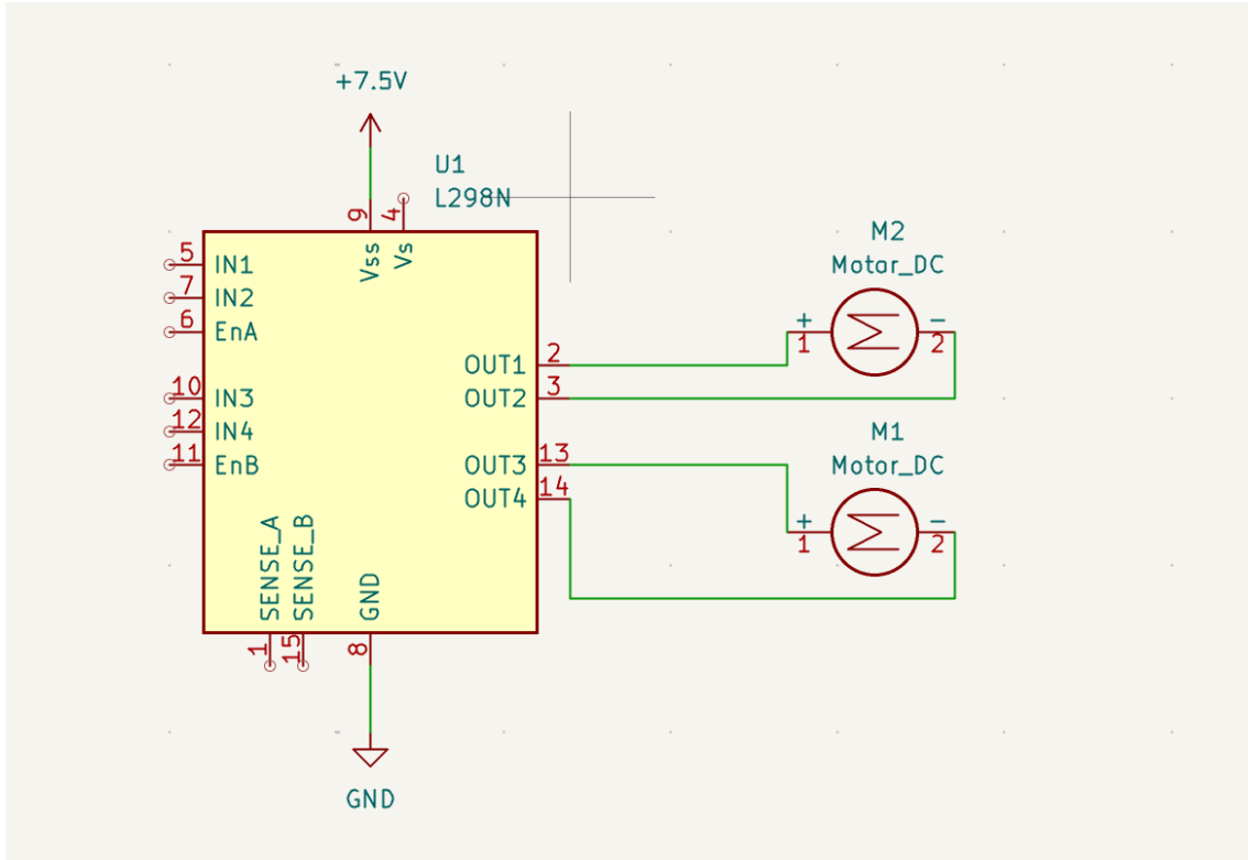
Figure 9: Diagram of connections between L298N with 2 6V TT gear motors
