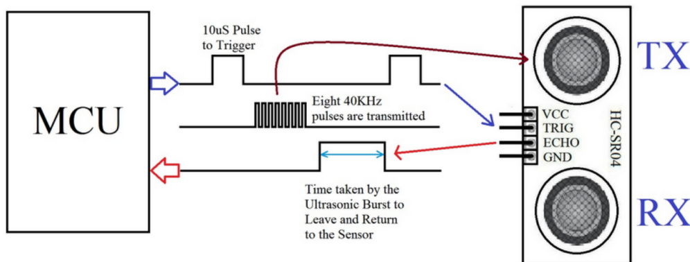
Figure 22: HC-SR04 timing schematic diagram
