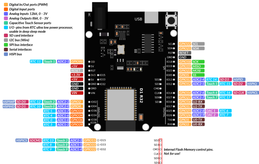
Figure 13: Wemos D1 R32 pins maps, more information about detailed pinout description in here
