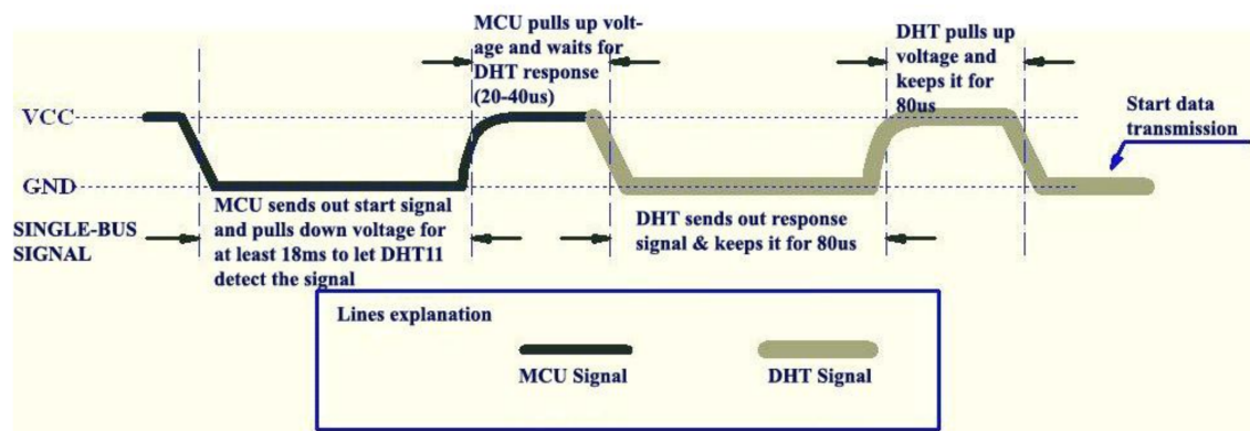
Figure 16: MCU Sends out Start Signal & DHT Responses
