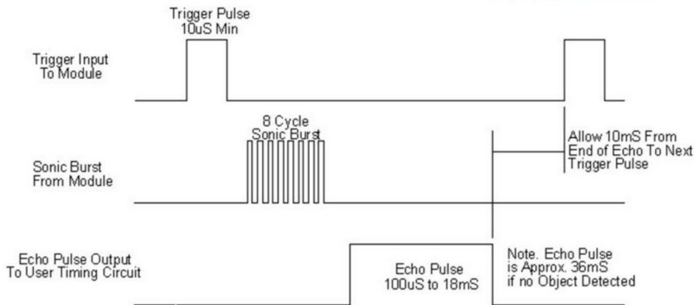
Figure 21: HC-SR04 timing schematic diagram
