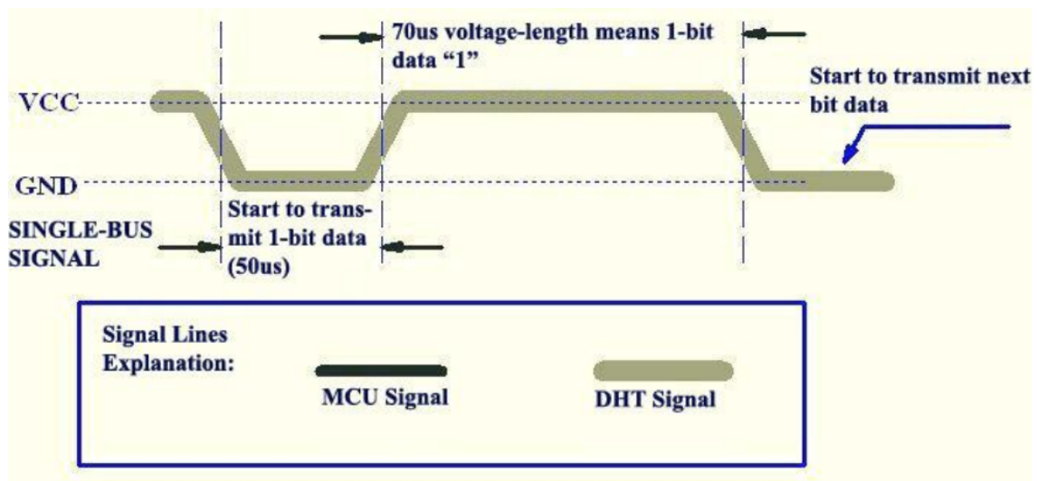
Figure 18: Data "1" Indication
