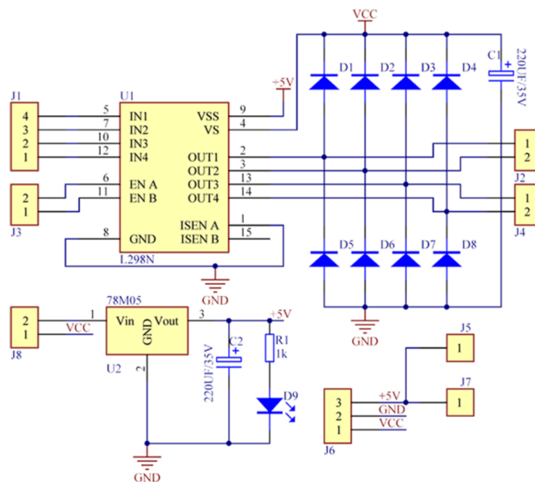
Figure 11: Schematic Diagram of L298N H-bridge DC motor driver
