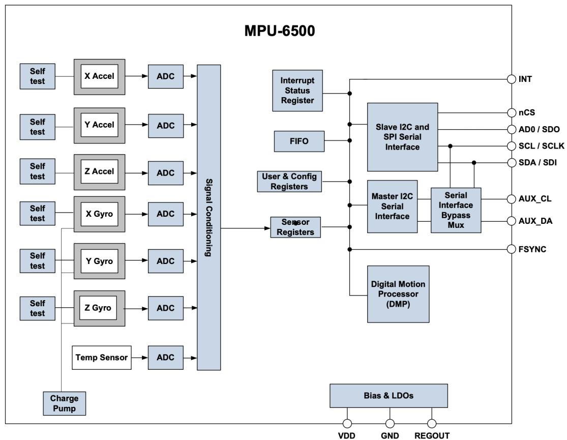
Figure 24: MPU-6500 block diagram, more information can be found in this datasheet , announced by TDK InvenSense
