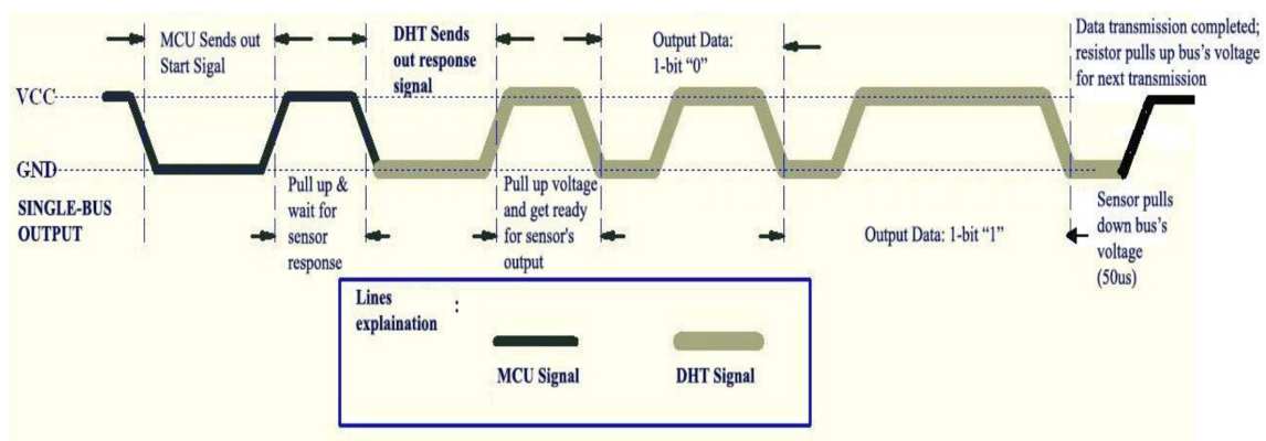
Figure 16: Detailed DHT 11 communication signal figure with MCU
