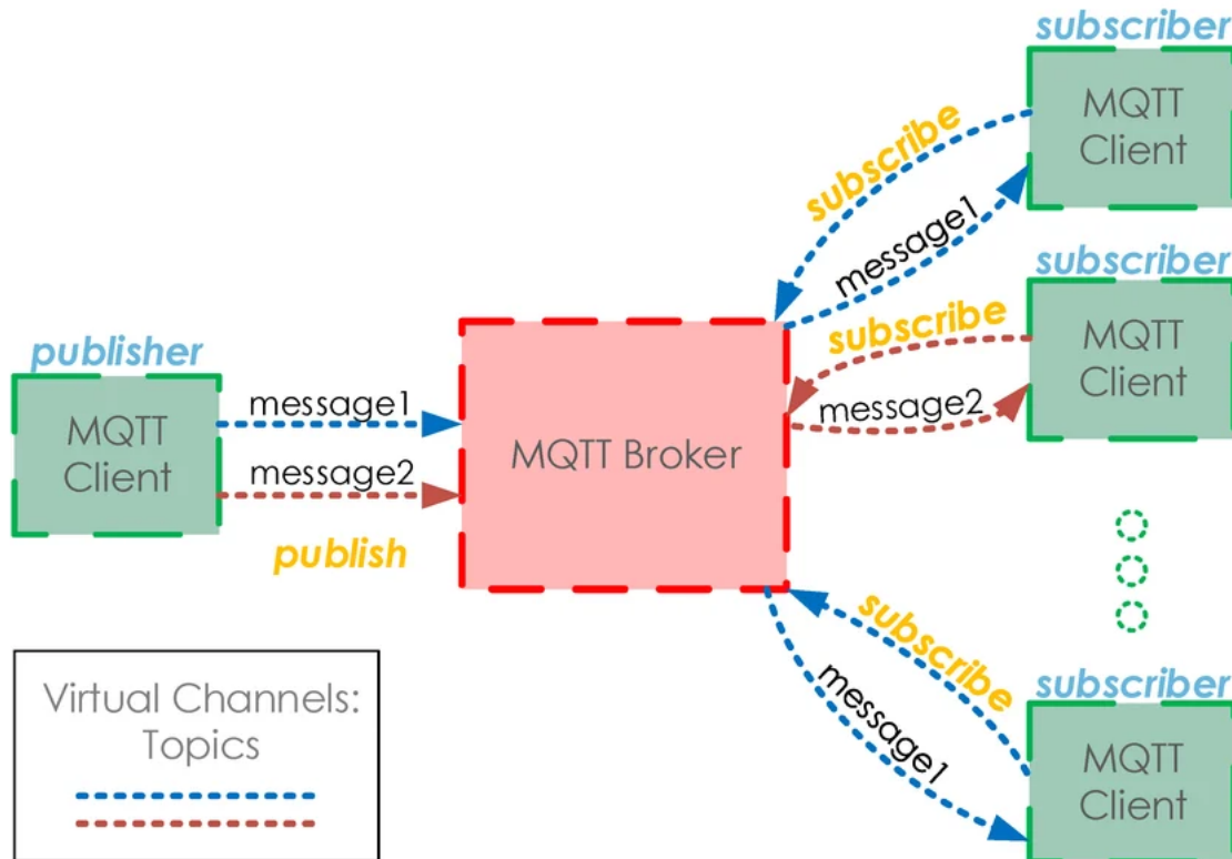
Figure 28: MQTT workflow diagram
