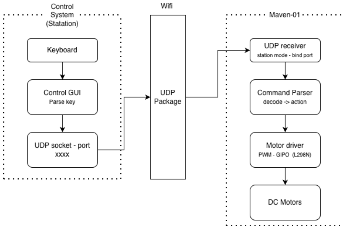
Figure 29: UDP control workflow diagram
