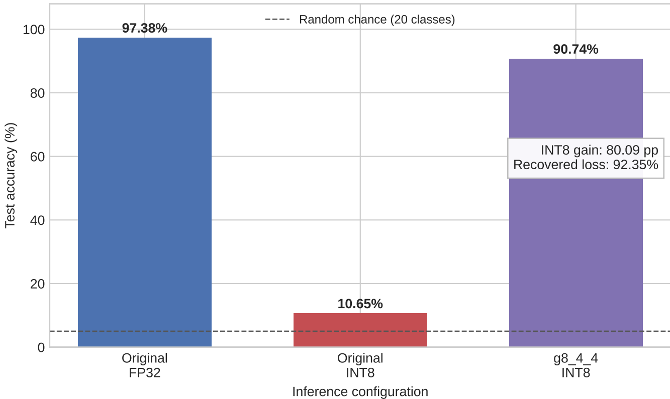
INT8 accuracy recovery with structural grouping
