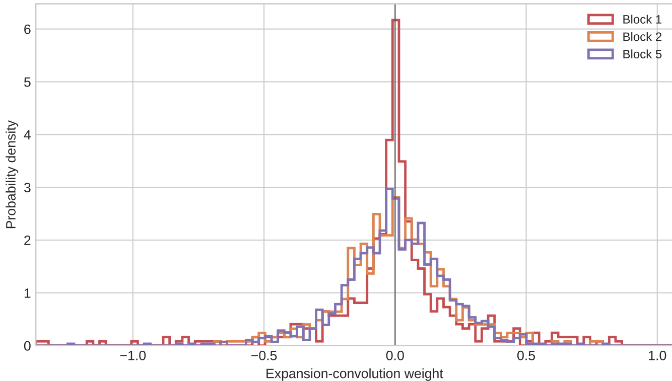
Weight distributions in the g8_4_4 blocks
