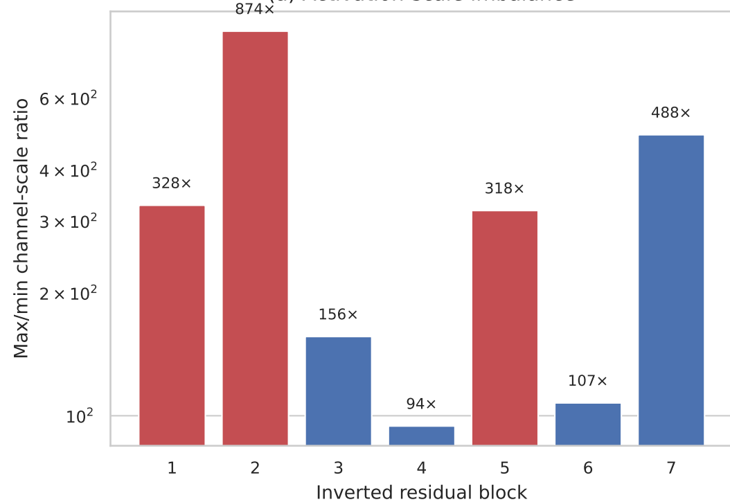
(a) Activation-scale imbalance
