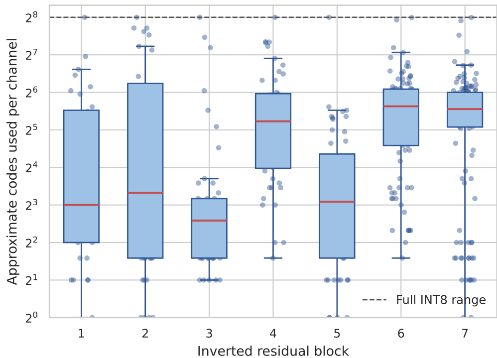
(b) Effective INT8-code utilization
