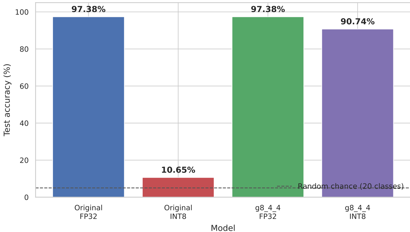
Effect of structural grouping on INT8 accuracy
