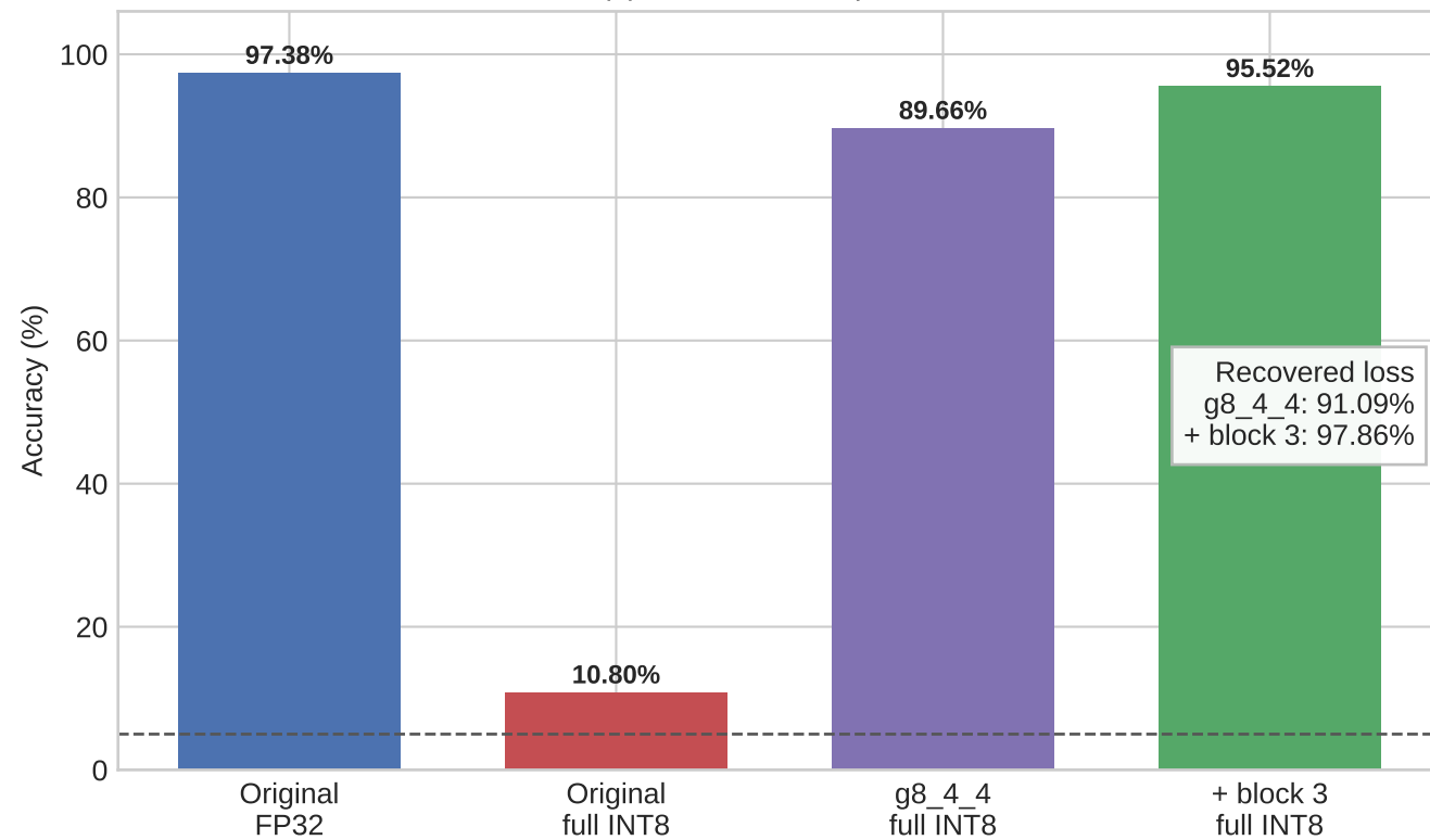
(a) Validation comparison
