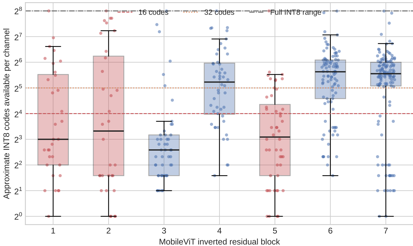
Per-channel utilization of the shared INT8 scale
