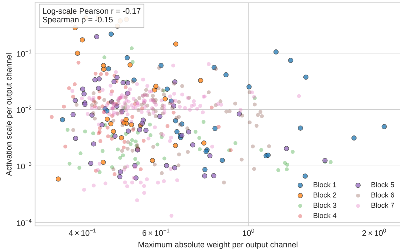
Association between filter magnitude and activation scale
