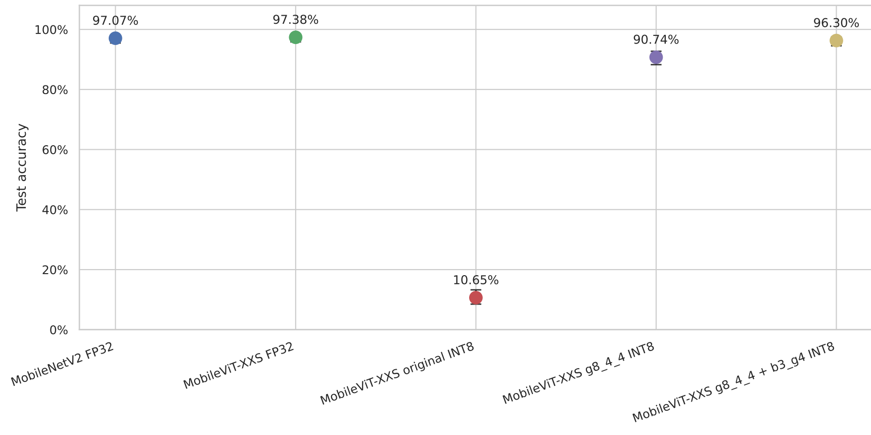
TFLite test accuracy with 95% Wilson confidence intervals
