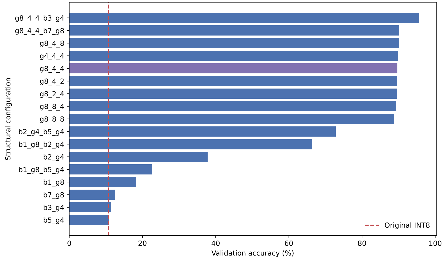
Validation accuracy across structural-grouping ablations
