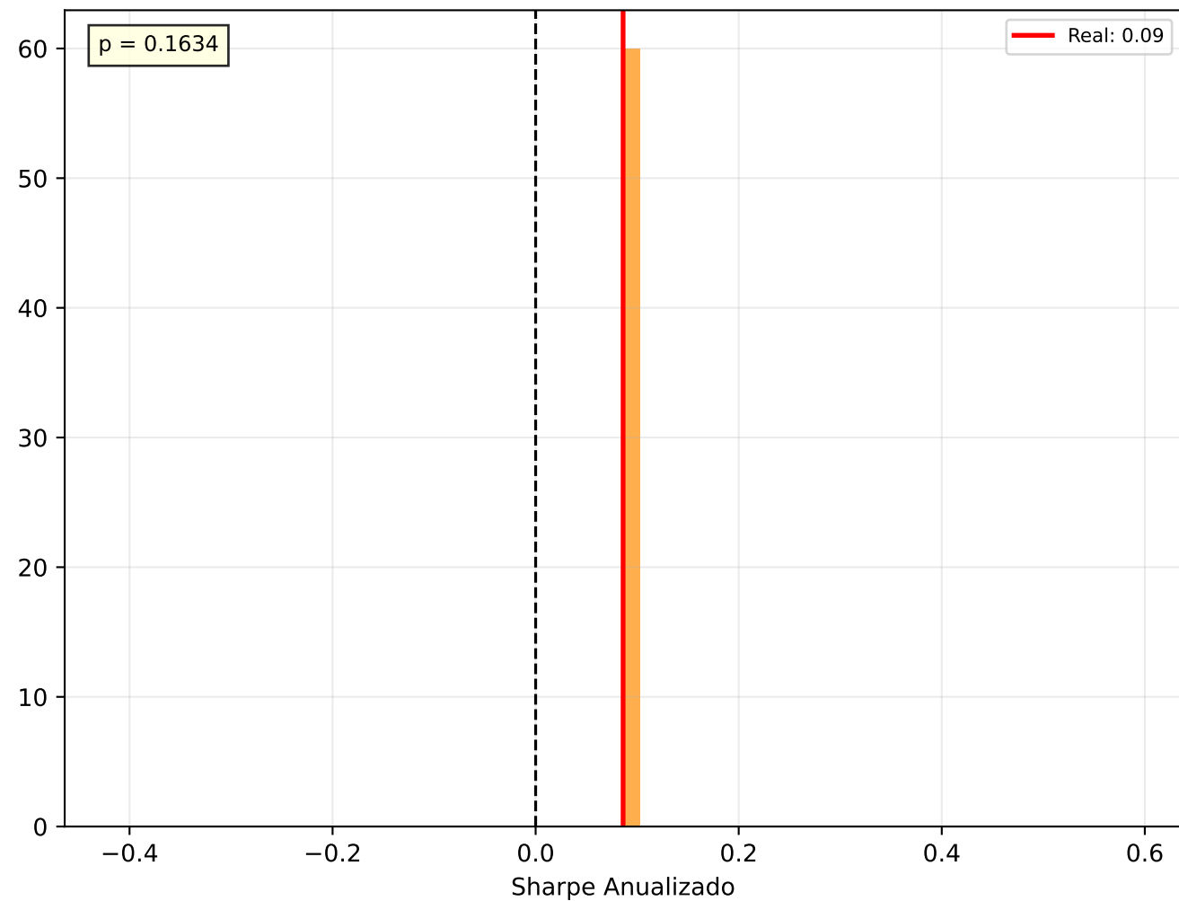
c) Monte Carlo — ABEV3.SA
