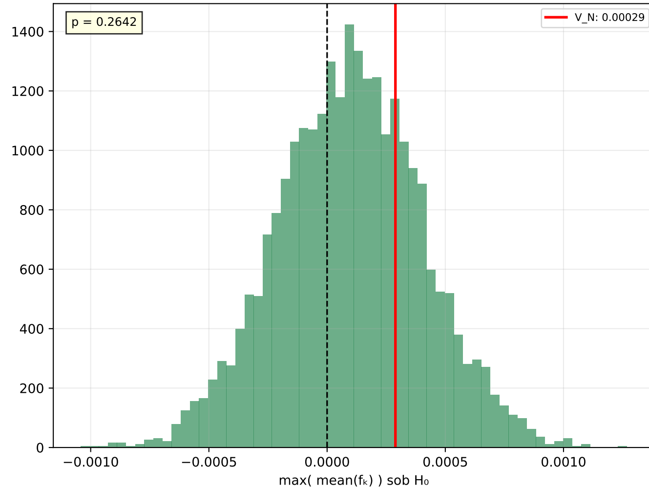
e) White's Reality Check — PETR4.SA
