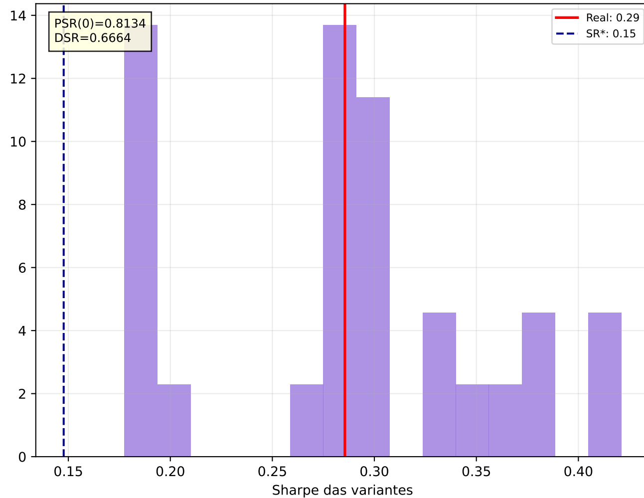
d) DSR — VALE3.SA
