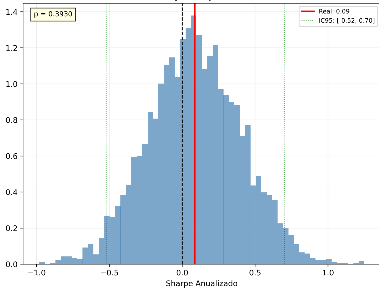
b) Bootstrap Sharpe — ABEV3.SA
