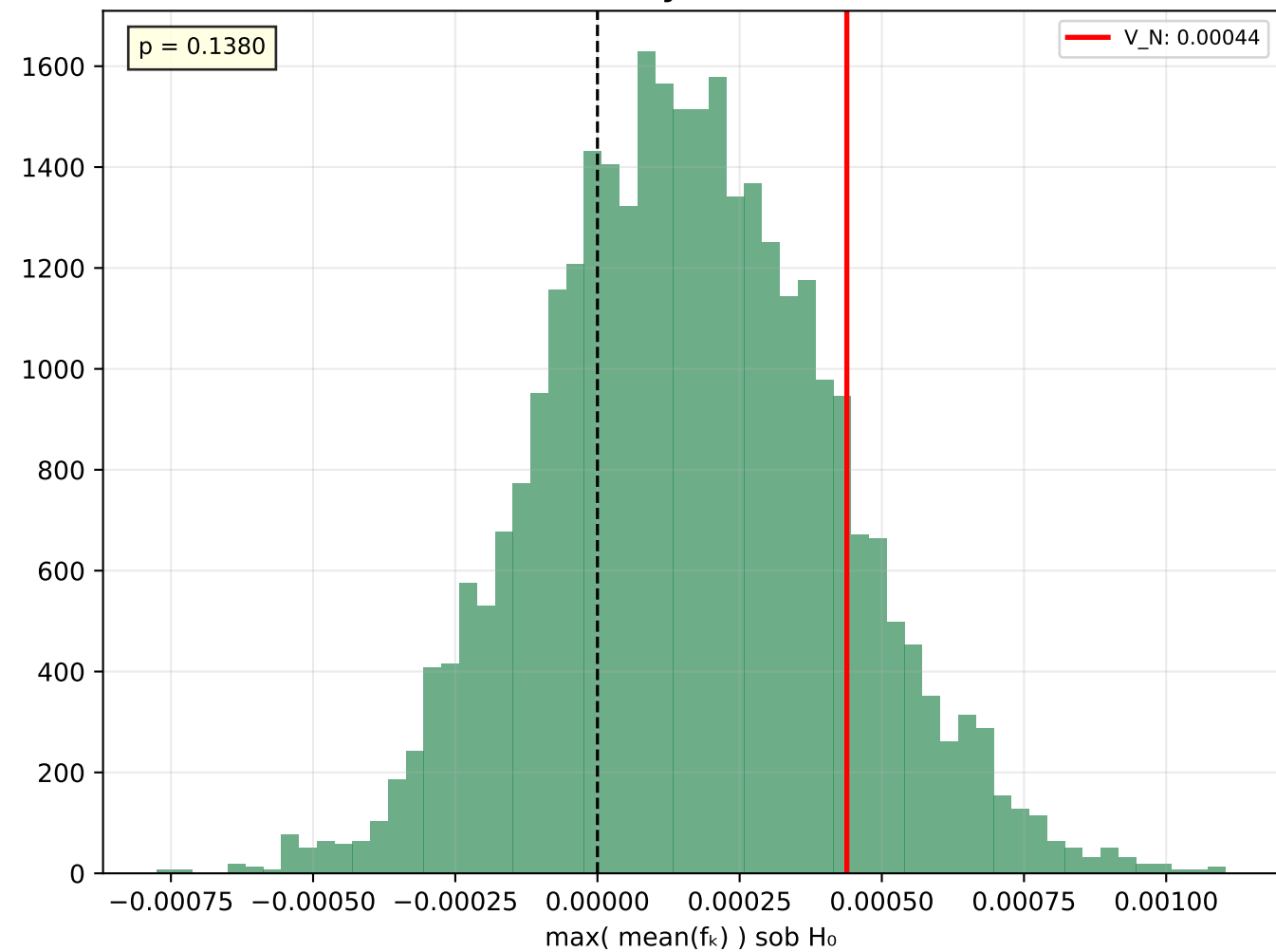
e) White's Reality Check — ITUB4.SA
