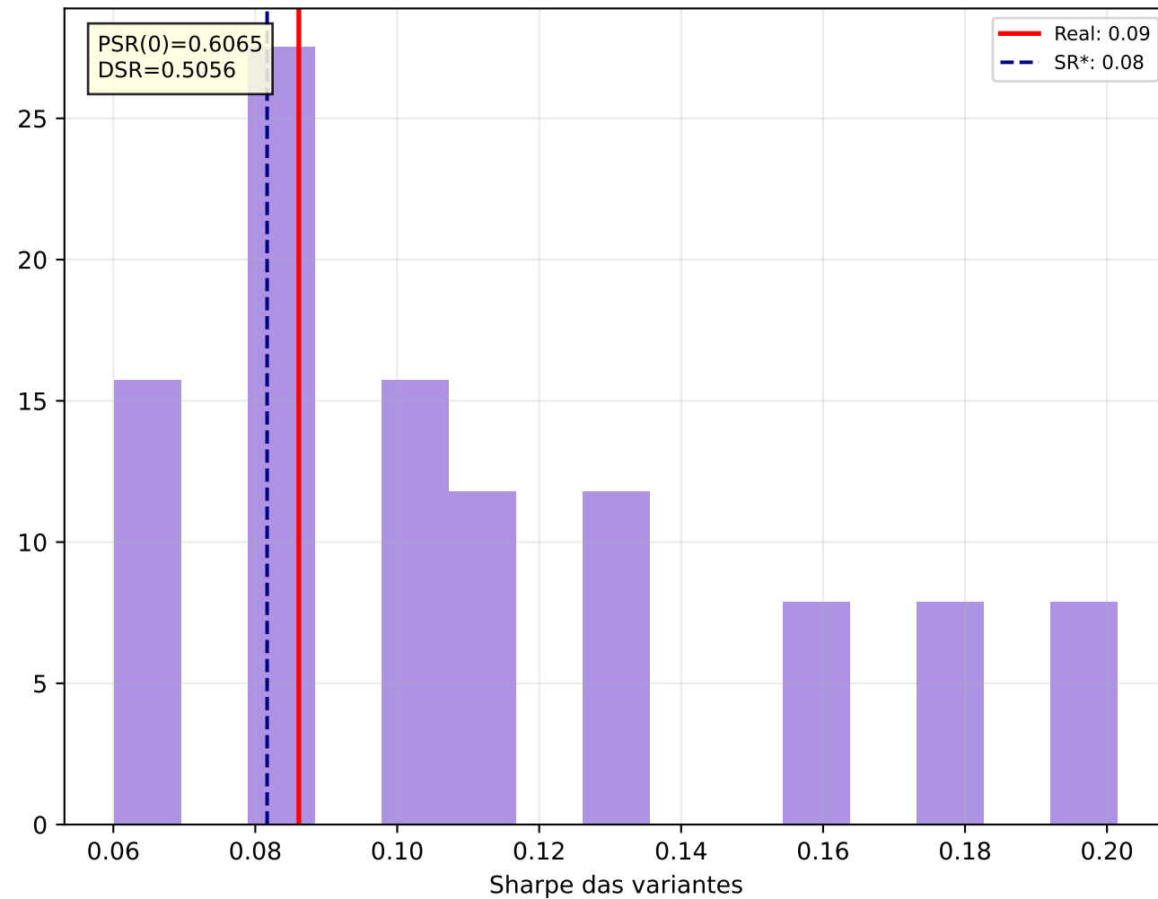
d) DSR — ABEV3.SA
