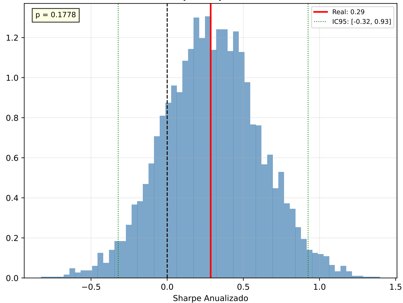
b) Bootstrap Sharpe — VALE3.SA
