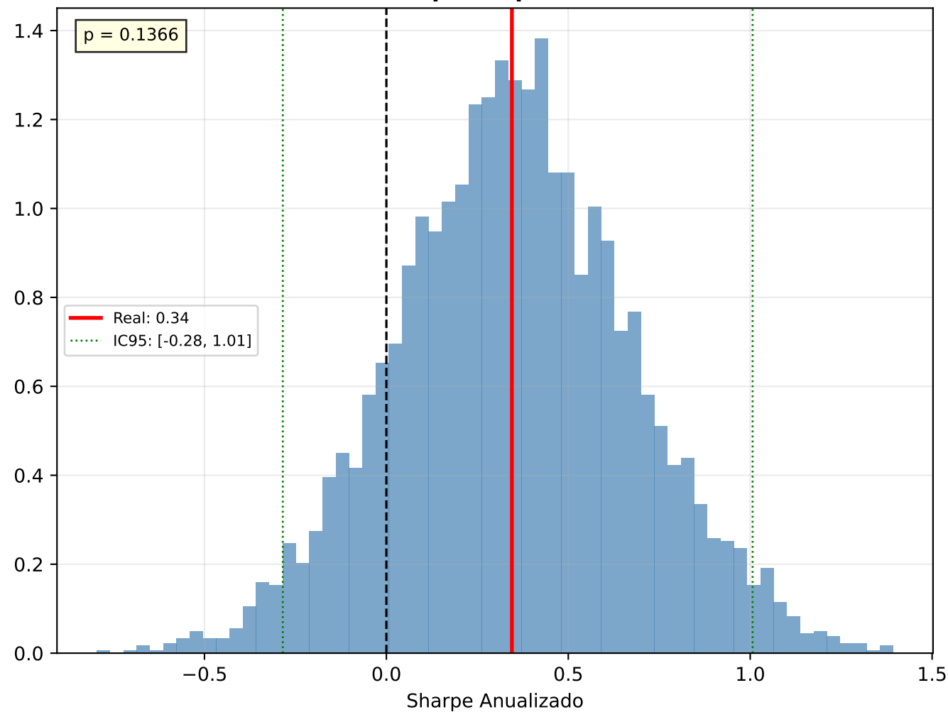
b) Bootstrap Sharpe — ITUB4.SA
