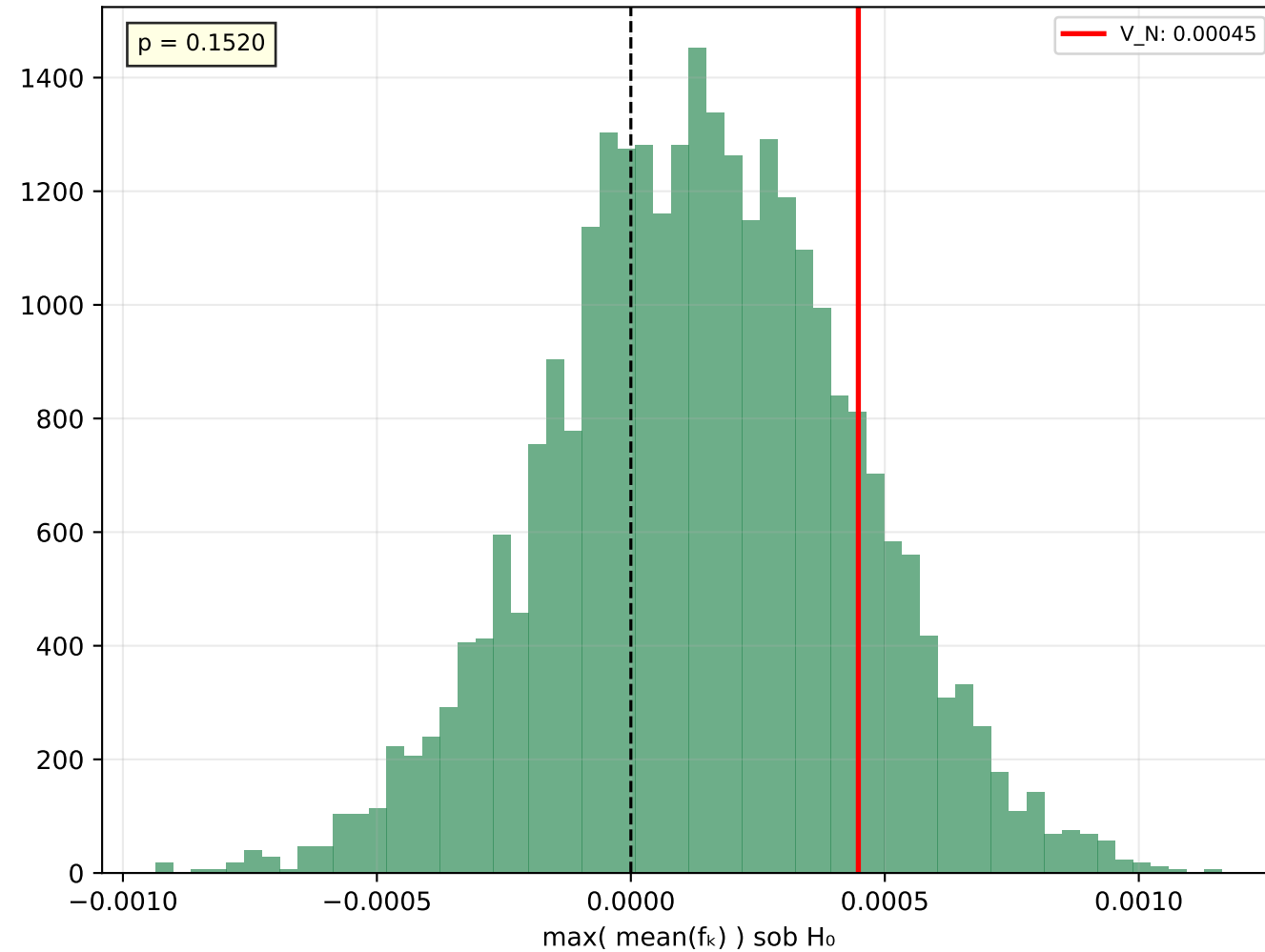
e) White's Reality Check — VALE3.SA
