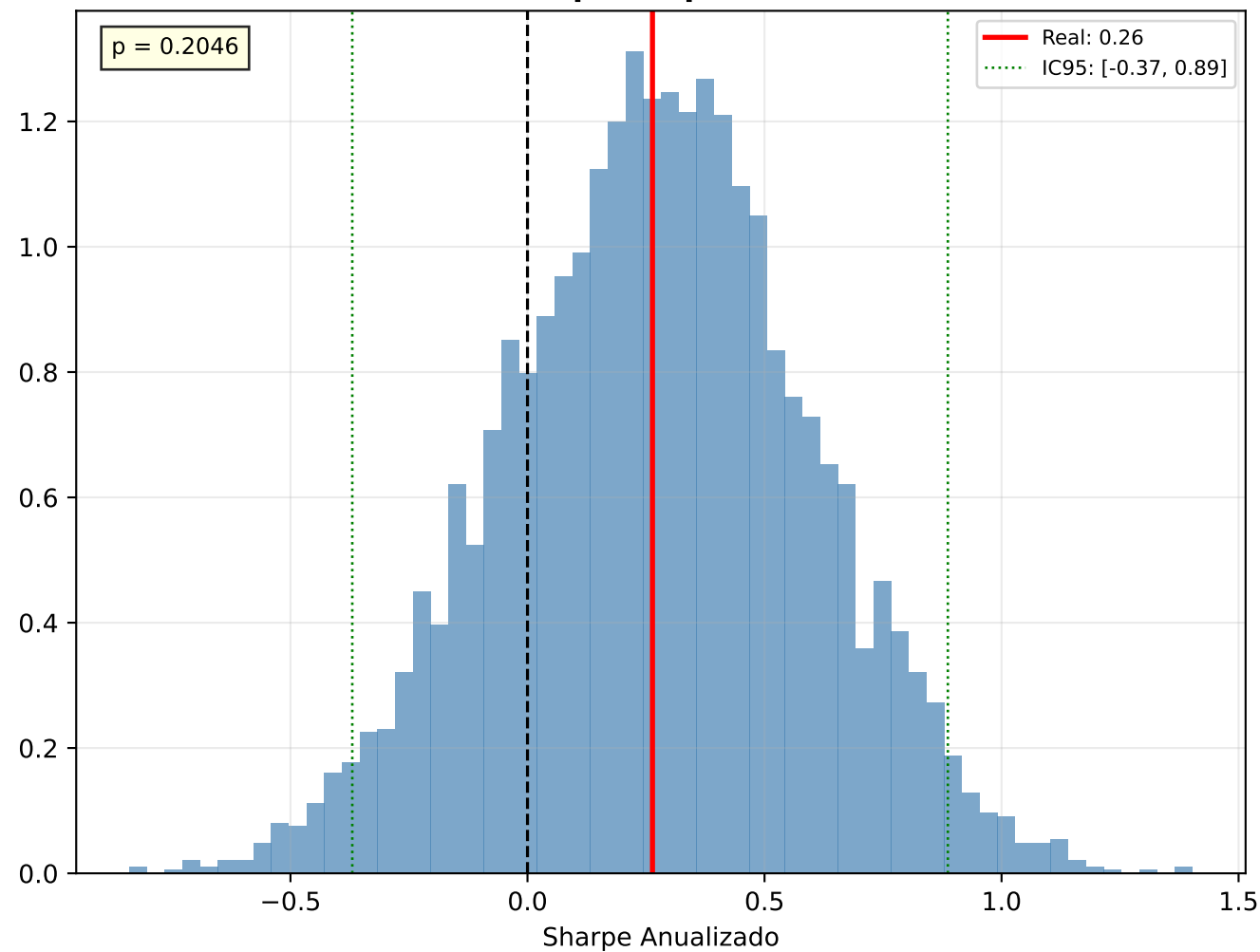
b) Bootstrap Sharpe — PETR4.SA
