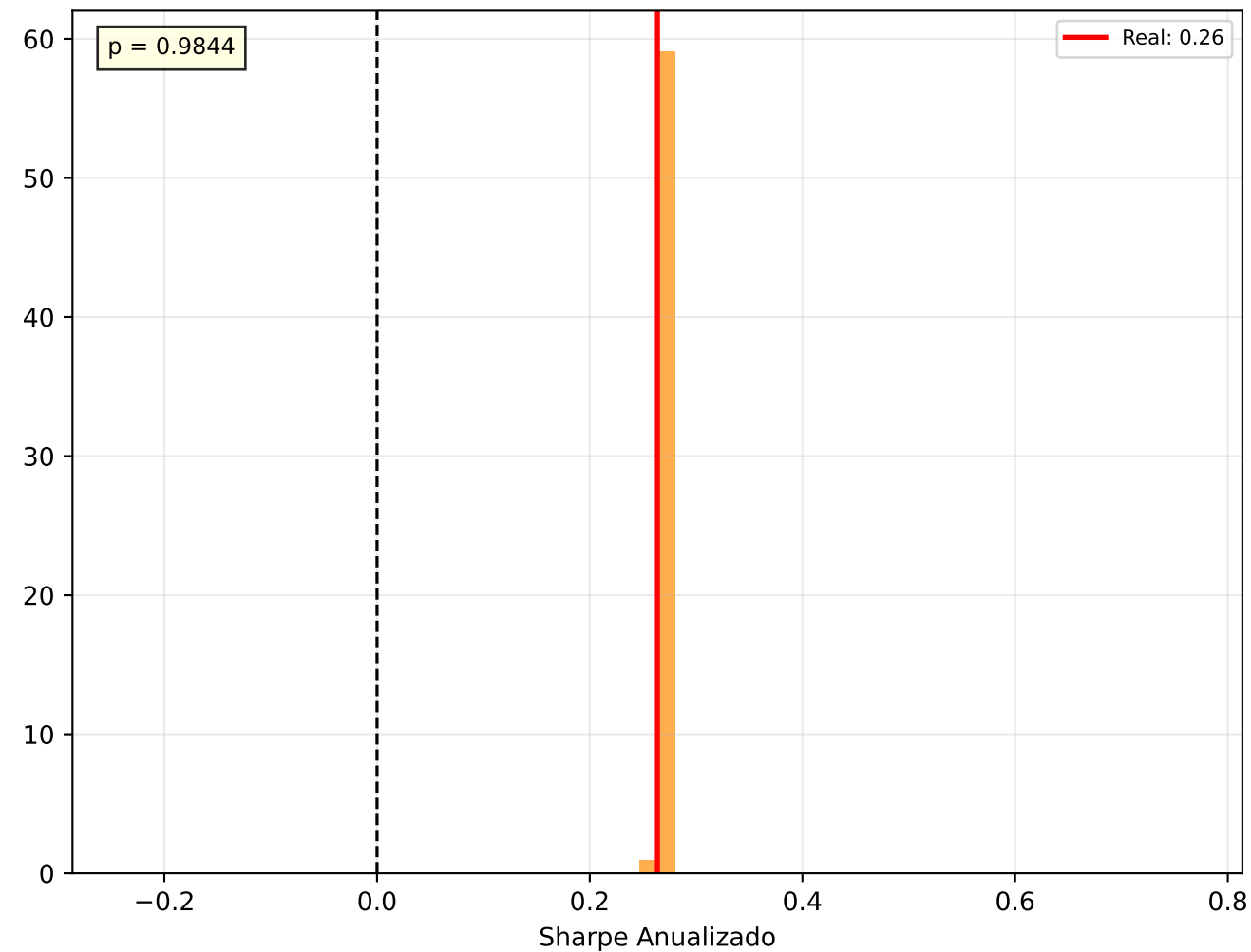
c) Monte Carlo — PETR4.SA
