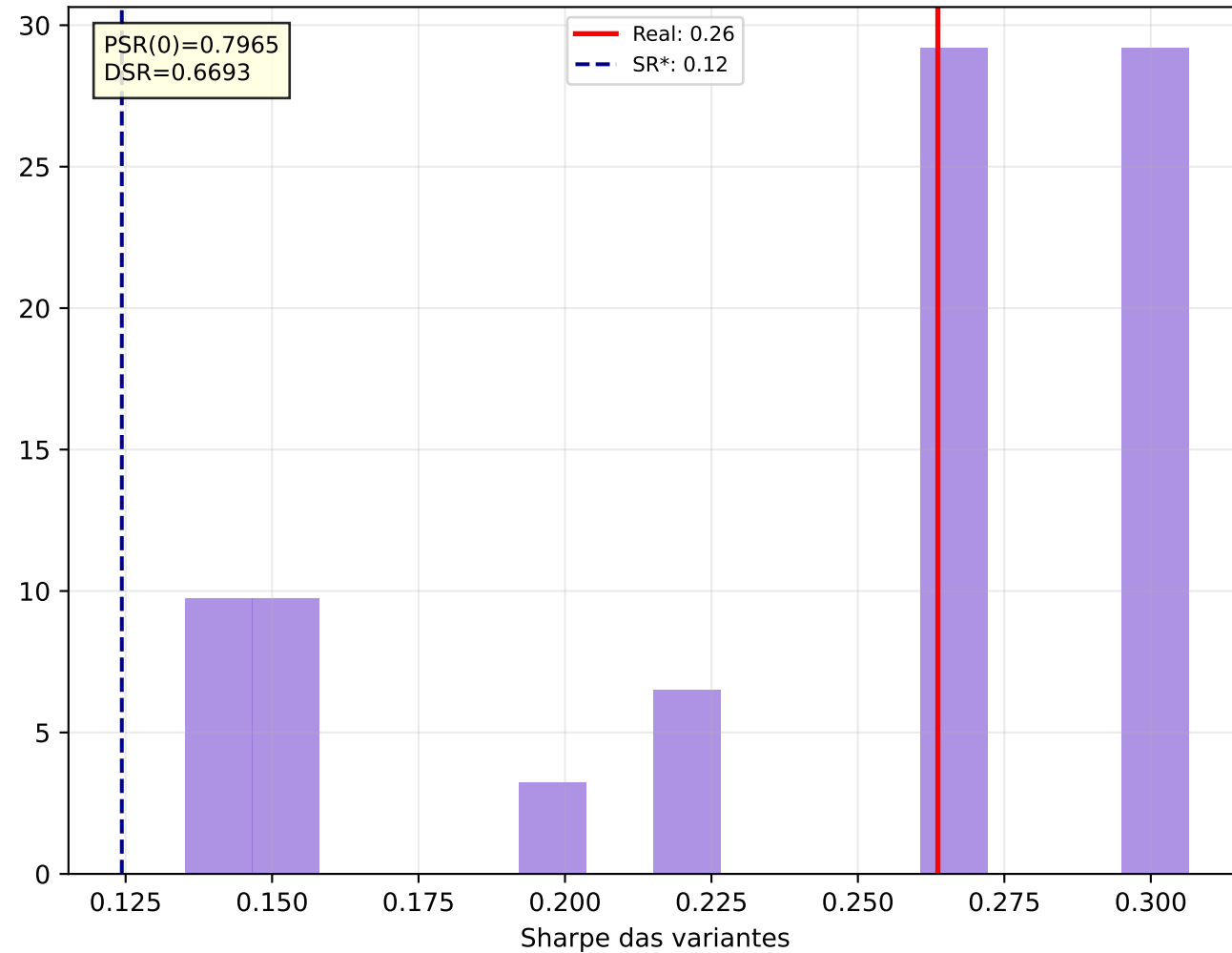
d) DSR — PETR4.SA
