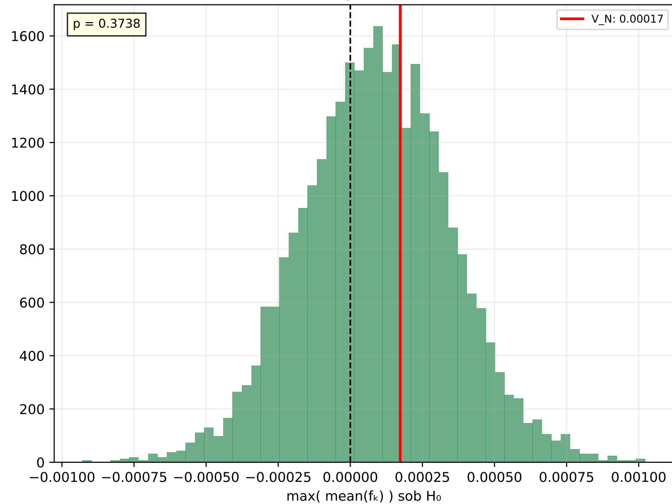
e) White's Reality Check — ABEV3.SA
