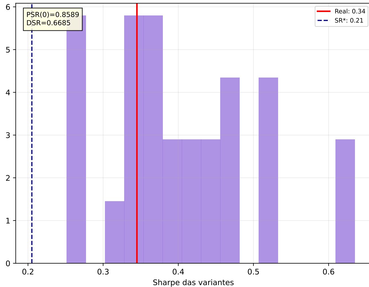
d) DSR — ITUB4.SA
