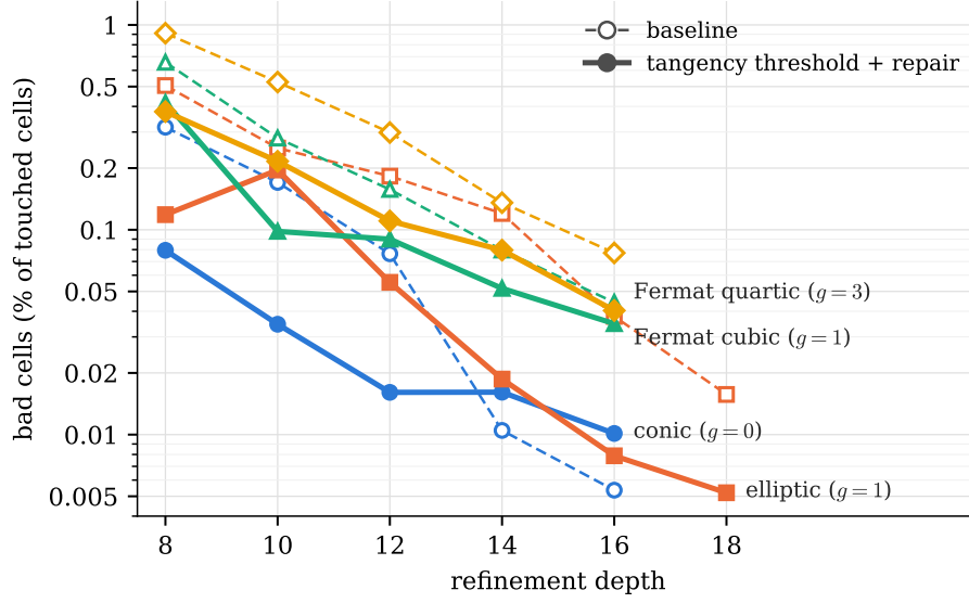
Figure 2: Percentage of touched cells whose extraction fails, against the refinement depth. Dashed lines with open markers: continuation alone. Solid lines: with tangency threshold 0.05 and two repair rounds.
