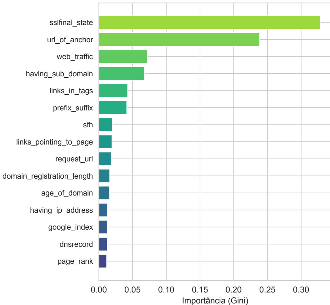
Top 15 Atributos — Random Forest
