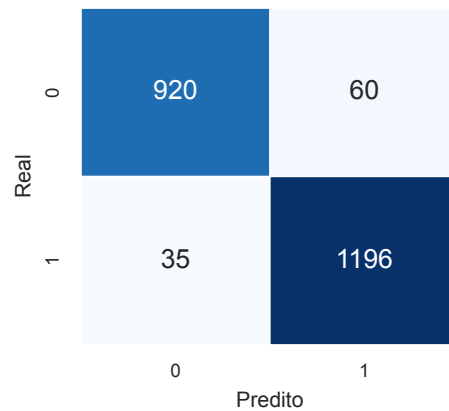
Gradient Boosting
