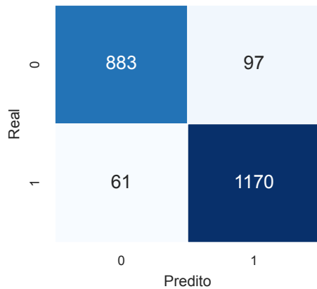
Random Forest
