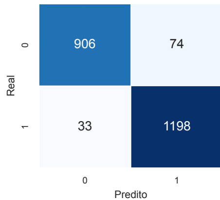
SVM RBF
