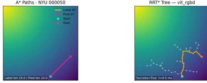
Figure 13: NYU planner overlays for the ViT RGBD model (scene 000050). The ViT maintains the corridor structure and produces a compact RRT* tree with minimal detours, illustrating its global context advantages.
