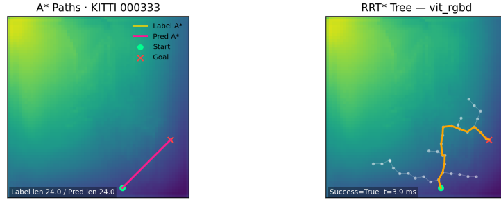
Figure 14: KITTI planner overlays for the ViT RGBD model (scene 000333). Slightly smoother A* trajectories and a wider RRT* tree highlight the remaining calibration gap relative to the UNet retrain in Figure 1.
