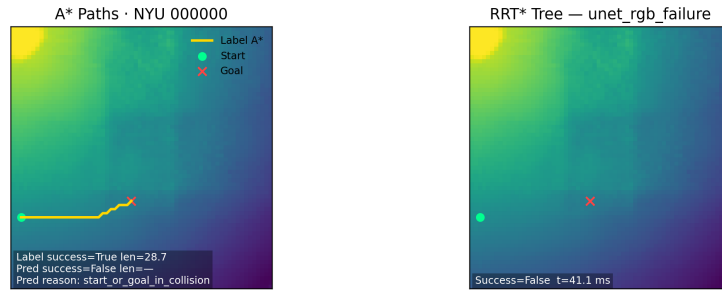
Figure 15: NYU failure-case overlay for the UNet RGB model (scene 000000). Labels provide a clean path, but the RGB-only prediction inflates the doorway and blocks A*. The RRT* tree terminates near the start, mirroring the logged planner failure.
