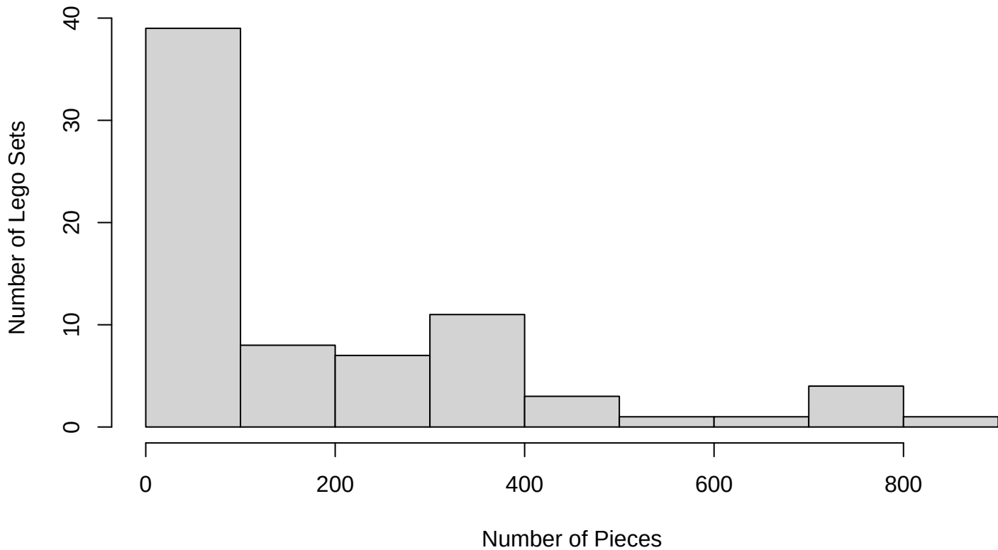
Histogram for Lego's Pieces
