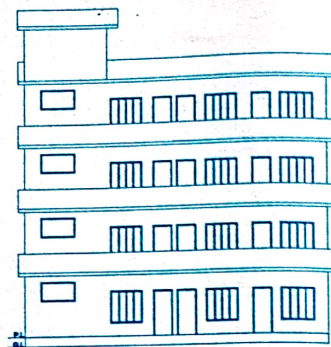
FRONT ELEVATION
