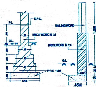
FOUNDATION & BOUNDARY DETAIL
