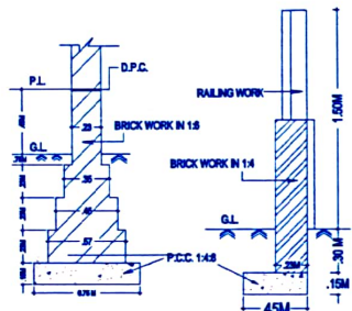
FOUNDATION & BOUNDARY DETAIL
