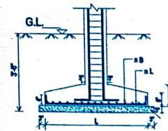
TYP. SECTION OF FOOTING
