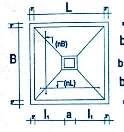
TYP. PLAN OF FOOTING
