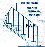
STAIR DETAIL
