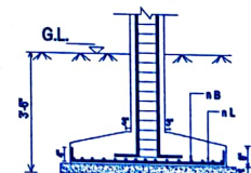
TYP. SECTION OF FOOTING
