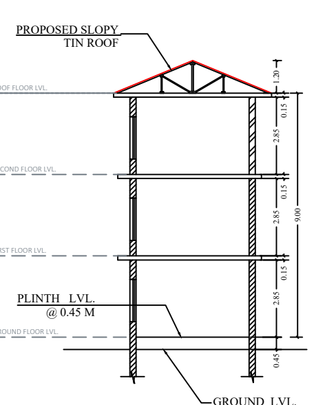
SECTION AT Y-Y' (COTTAGE)
