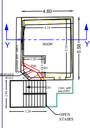
SANCTIONED / EXISTING SECOND FLOOR PLAN (COTTAGE)
