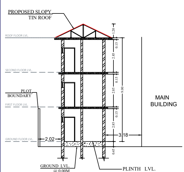
SECTION AT A-A' (BUILDING - 2)
