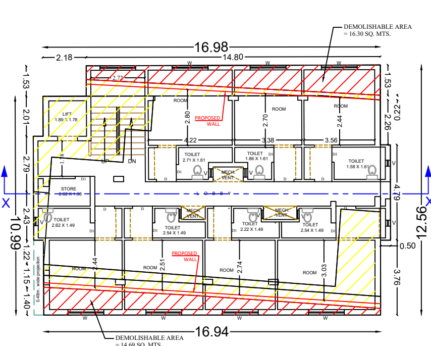
SANCTIONED / EXISTING SECOND FLOOR PLAN (MAIN BUILDING)
