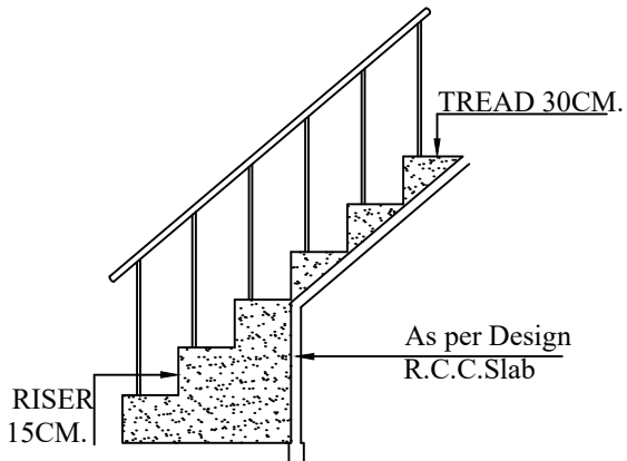
STAIRS DETAILS
