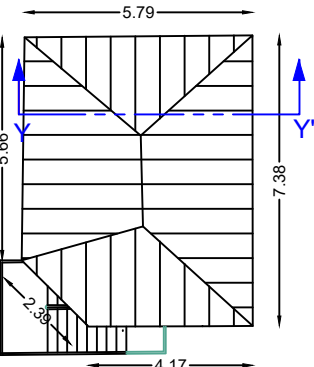
SLOPY ROOF PLAN (COTTAGE)
