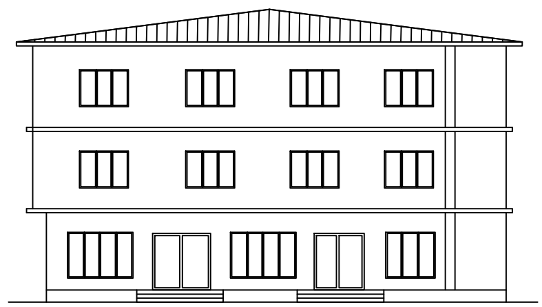
FRONT ELEVATION - MAIN BUILDING
