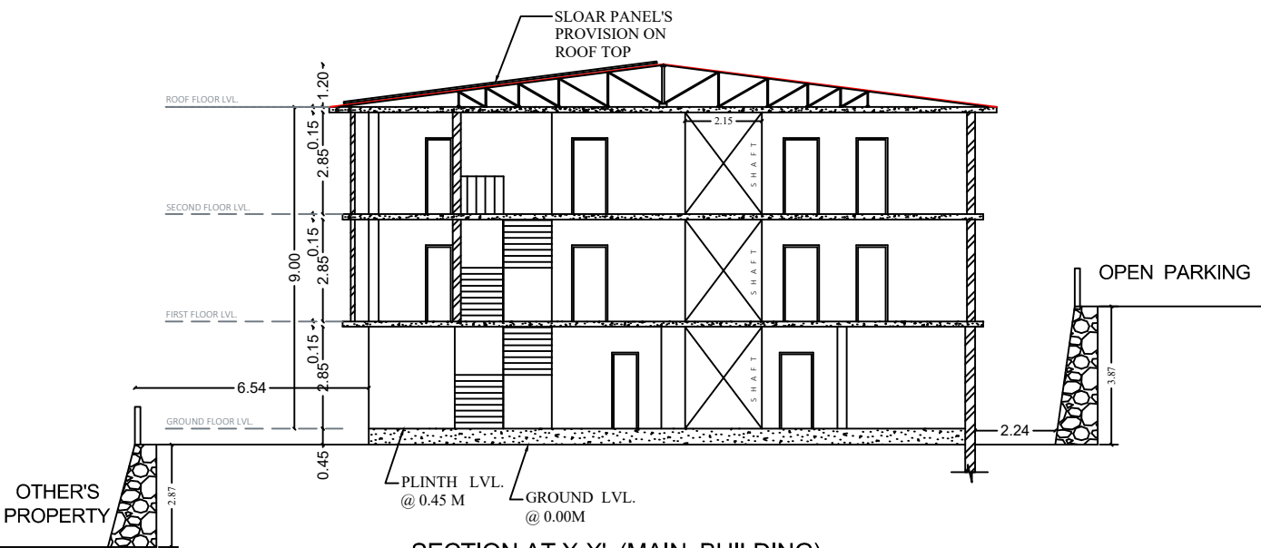
SECTION AT X-X' (MAIN BUILDING)
