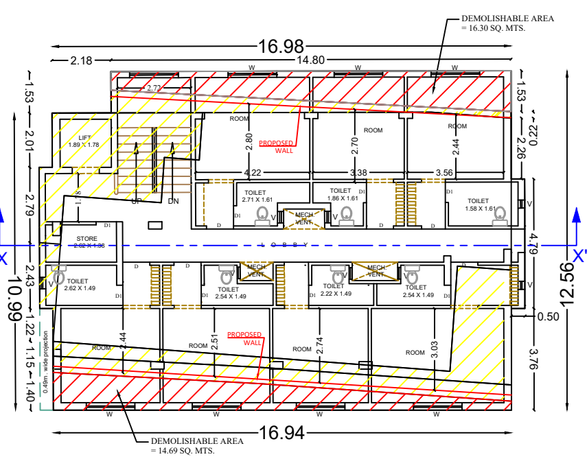
SANCTIONED / EXISTING FIRST FLOOR PLAN (MAIN BUILDING)
