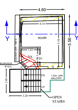
SANCTIONED / EXISTING FIRST FLOOR PLAN (COTTAGE)
