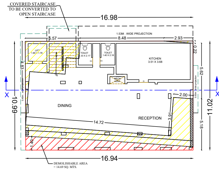
SANCTIONED / EXISTING GROUND FLOOR PLAN (MAIN BUILDING)
