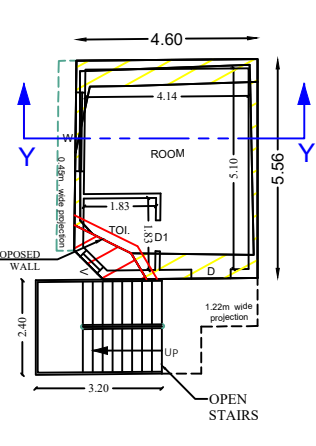
SANCTIONED / EXISTING GROUND FLOOR PLAN (COTTAGE)
