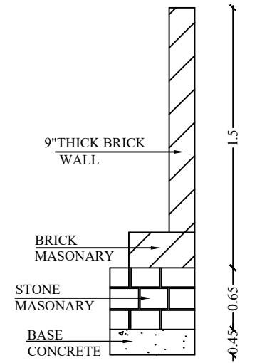
BAOUNADRY WALL DETAILS
