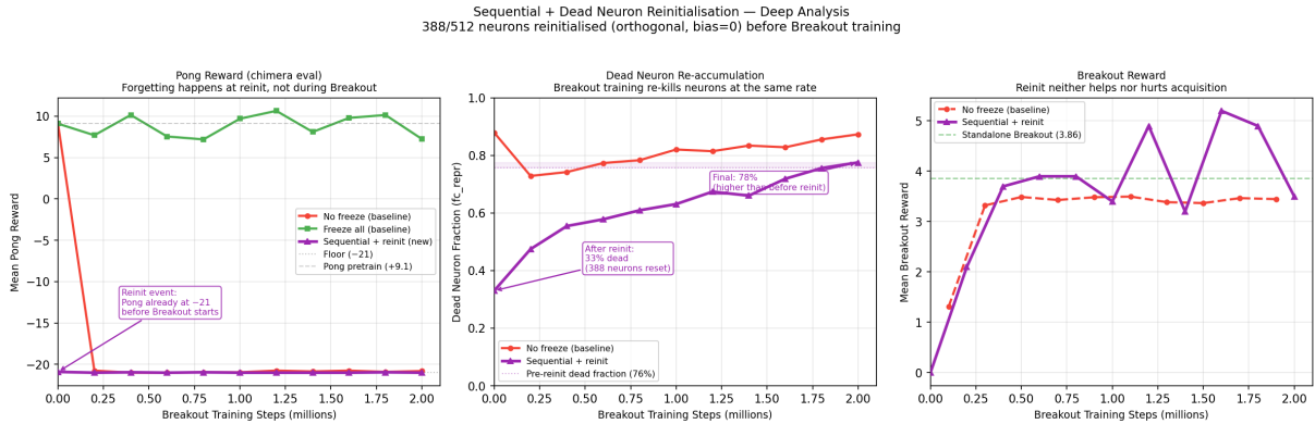
Figure 1: Sequential + Dead Neuron Reinitialisation. Left: Pong reward is already at floor before any Breakout training — forgetting occurs at reinit, not during Breakout. Centre: dead neurons drop from 76% to 33% at reinit then climb back to 77.5% over 2M Breakout steps. Right: Breakout reward is identical to the no-freeze baseline — reinit neither helps nor hurts new task acquisition.
