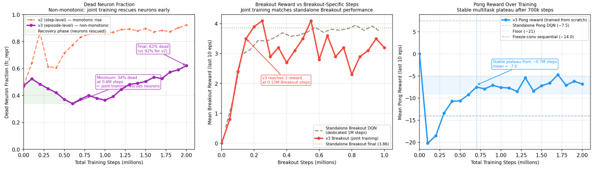
Figure 2: Interleaved v3 deep dive. Left: dead neuron fraction drops during the first 600k steps (joint gradients rescue neurons) then rises during re-specialisation. Centre: v3 Breakout reward vs Breakout-specific steps, reaching standalone Breakout performance in \sim 150k steps vs 2M for the dedicated DQN. Right: Pong reward stabilises around -7 from 700k steps onwards.
