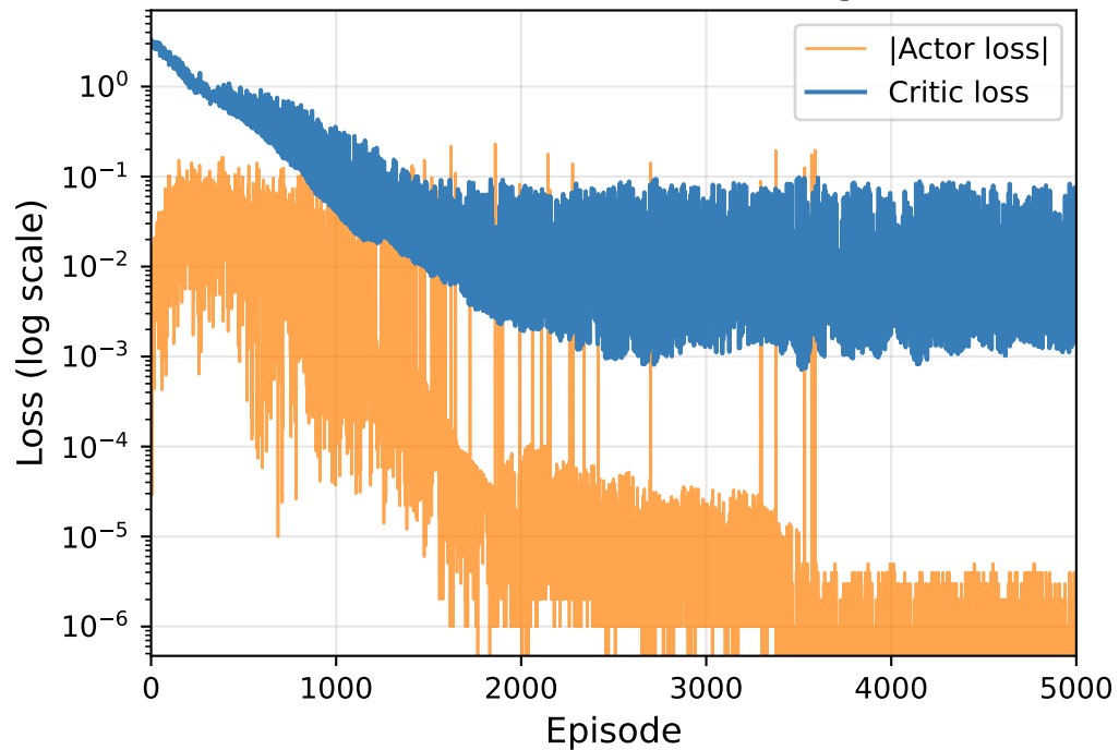
A2C v3: Actor Loss \rightarrow 0 (Zero-Advantage Fixed Point)
