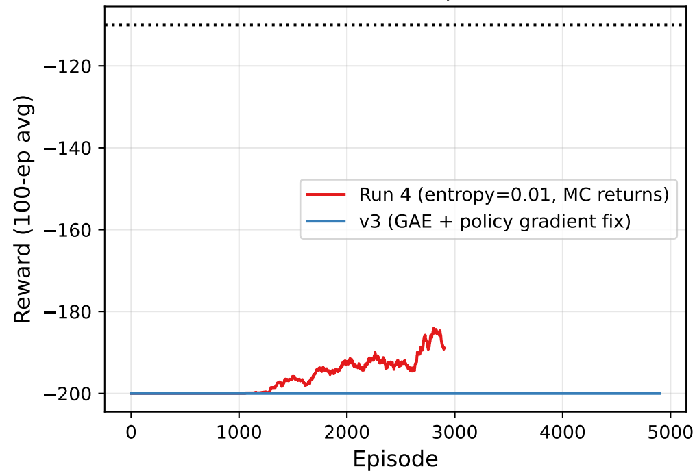
A2C: Best vs Fixed Implementation
