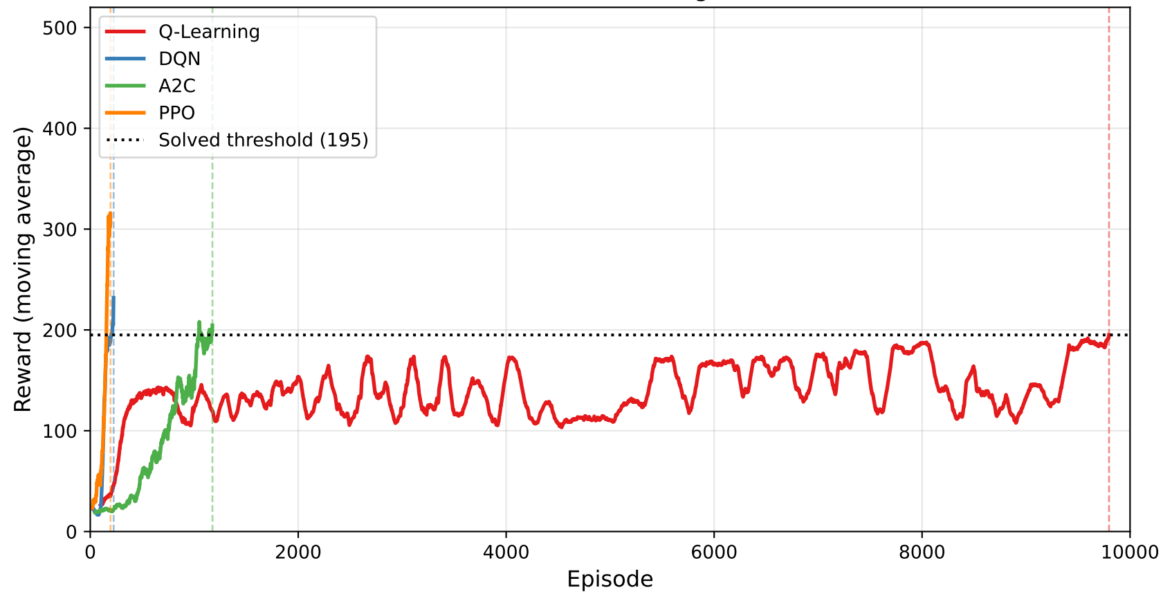
CartPole-v1: All Four Algorithms
