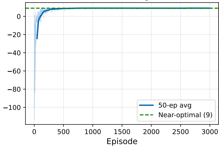
GridWorld Q-Learning: Reward
