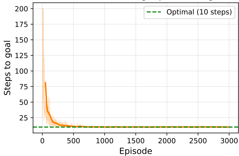
GridWorld Q-Learning: Episode Length
