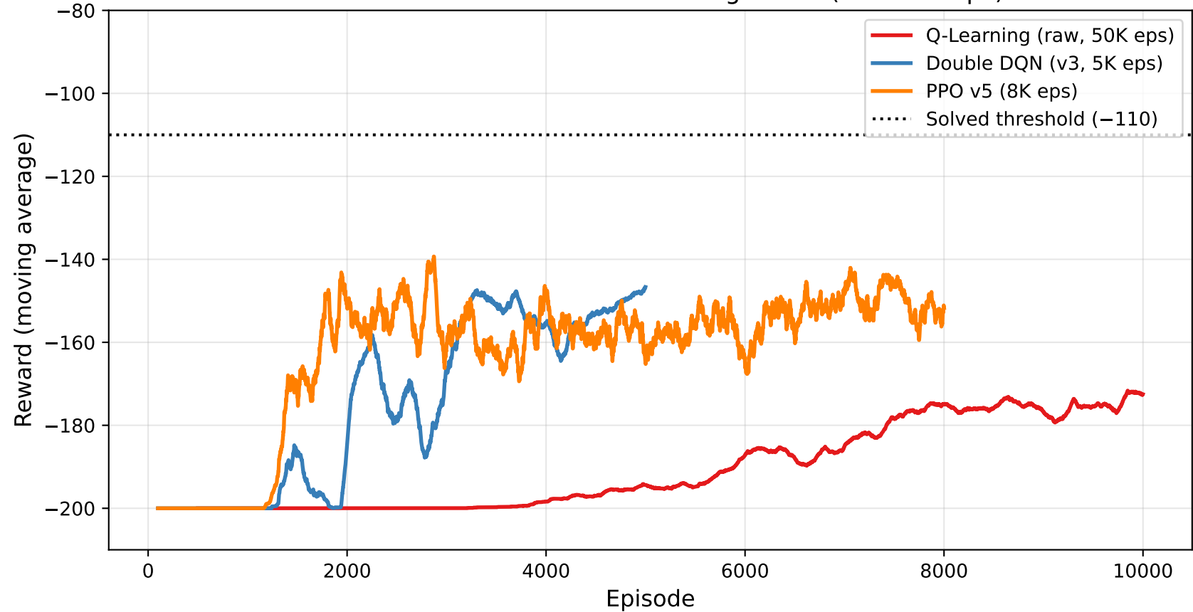
MountainCar-v0: Best Result Per Algorithm (first 10K eps)
