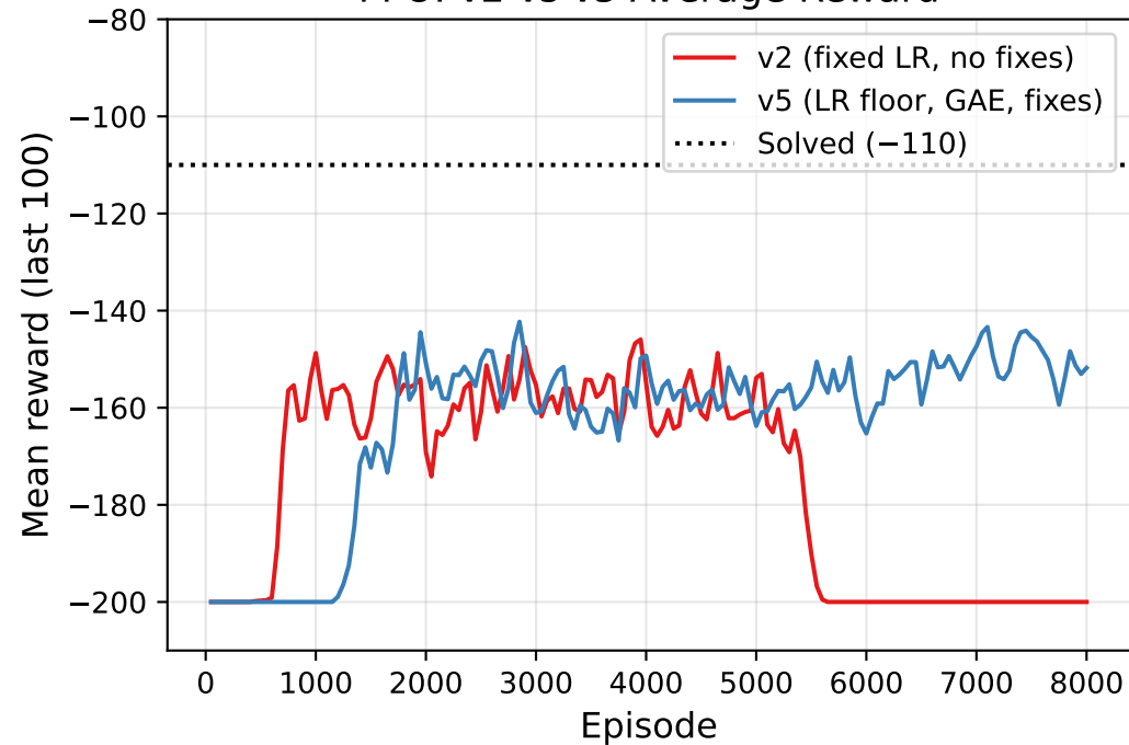
PPO: v2 vs v5 Average Reward
