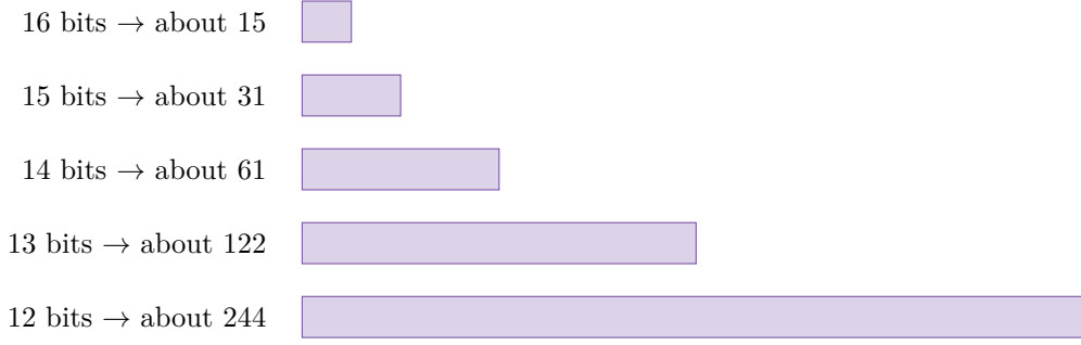
Figure 14: Under the independent 50/50-bit model, removing one prefix bit doubles the expected matching count.
