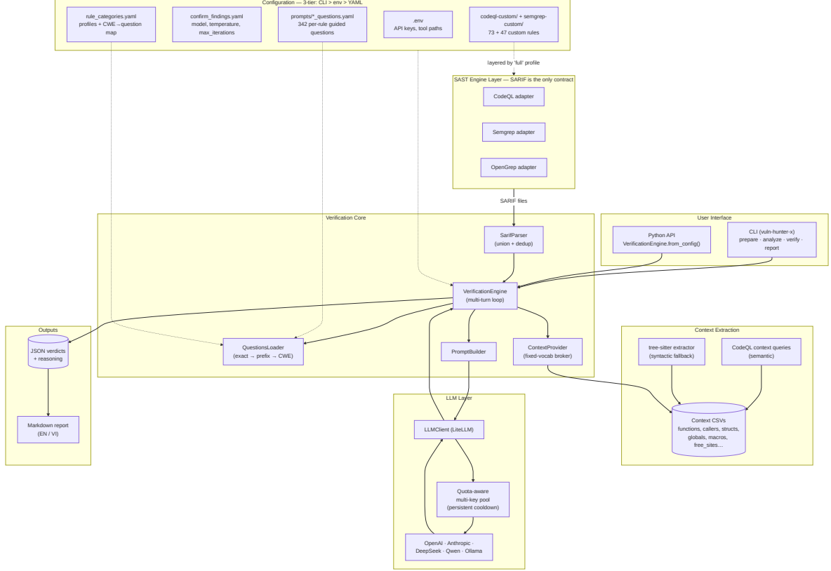
Figure 1: VulnHunterX framework architecture. SARIF acts as the sole contract between SAST engine adapters (CodeQL, Semgrep, OpenGrep) and the verification core. Context CSVs — extracted by CodeQL queries with a tree-sitter fallback — feed the multi-turn LLM verification loop without re-running the underlying SAST engine.
