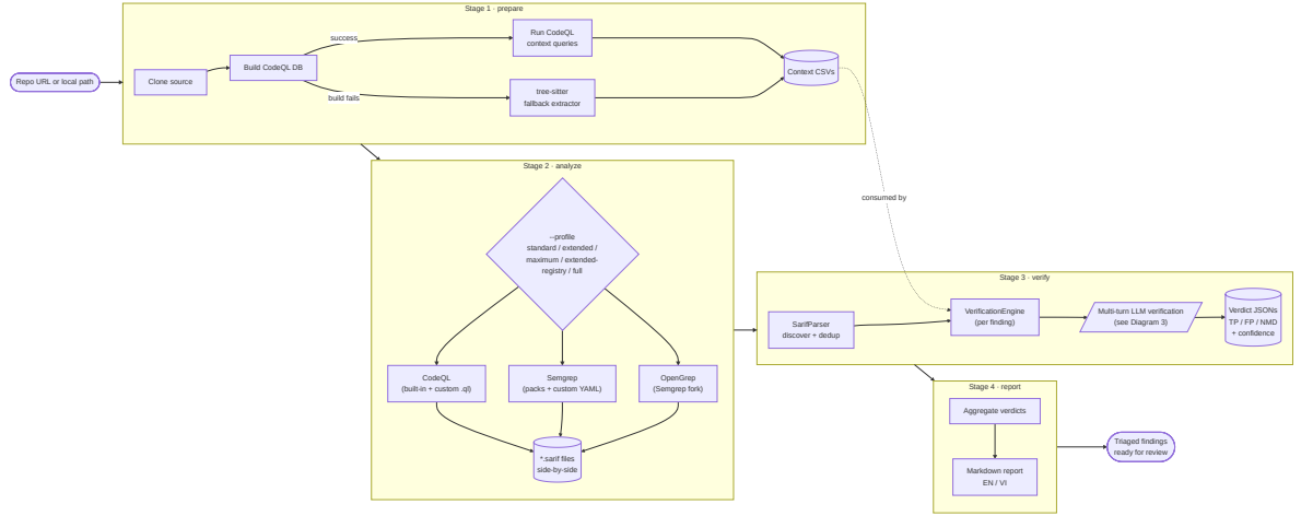
Figure 3: End-to-end pipeline (fuzzing stages excluded). Stage 1 prepares the repository (clone, CodeQL DB, context CSVs with tree-sitter fallback); Stage 2 runs CodeQL / Semgrep / OpenGrep gated by a profile ( standard , extended , maximum , extended-registry , full ) that controls custom-rule layering; Stage 3 dispatches each SARIF finding through the multi-turn LLM verifier of Figure 2; Stage 4 aggregates verdicts into a markdown report.
