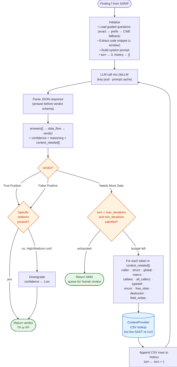
Figure 2: Per-finding LLM verification flow. The answer-before-verdict schema, the citation-based confidence downgrade, the fixed-vocabulary CSV broker, and the min_iterations / max_iterations loop guard. TP/FP terminate; NMD fetches additional context and re-enters the loop until budget exhaustion.
