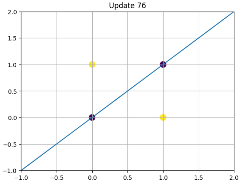
Figure 10: Decision boundary for XOR gate
