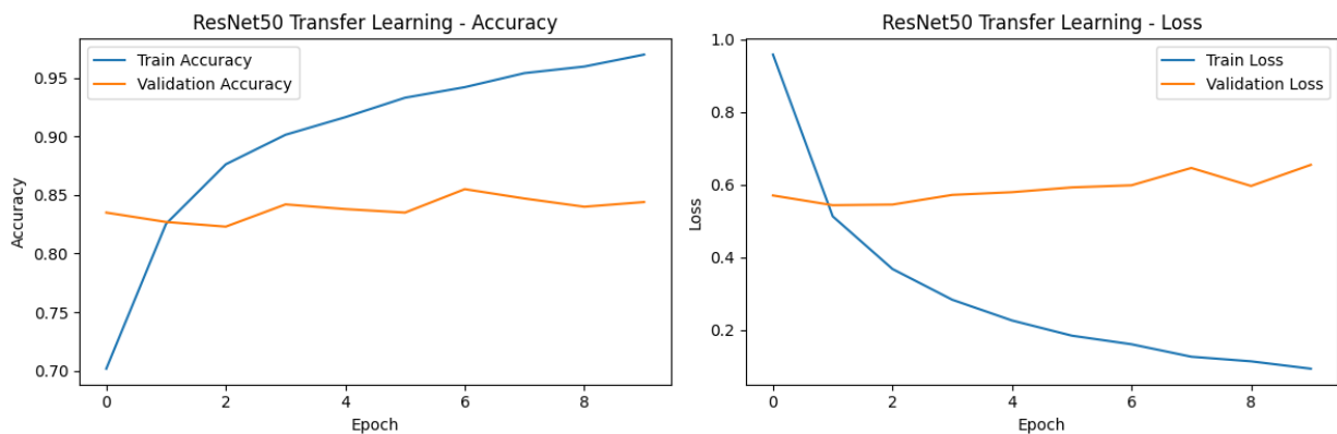
Figure: ResNet50 Transfer Learning – Training and Validation Accuracy/Loss
