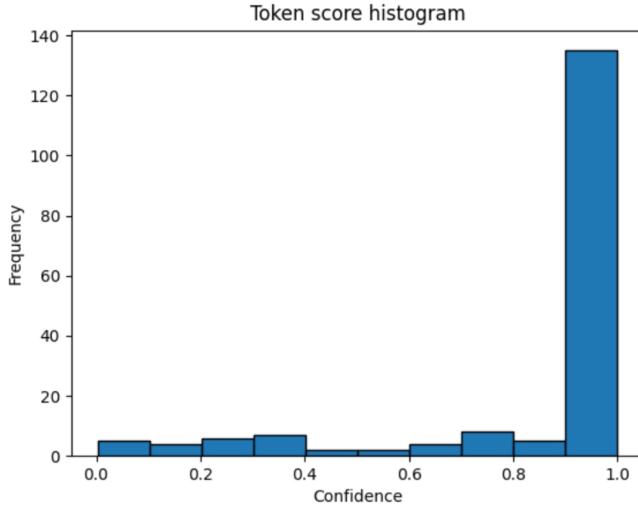
Figure 3.5: A Histogram that displays the distribution of the token confidence in the humaneval task 19. The confidence is displayed on the x-axis and the number tokens in each bin are on the y-axis. It can be seen that the model is mostly overconfident in its token selection.
